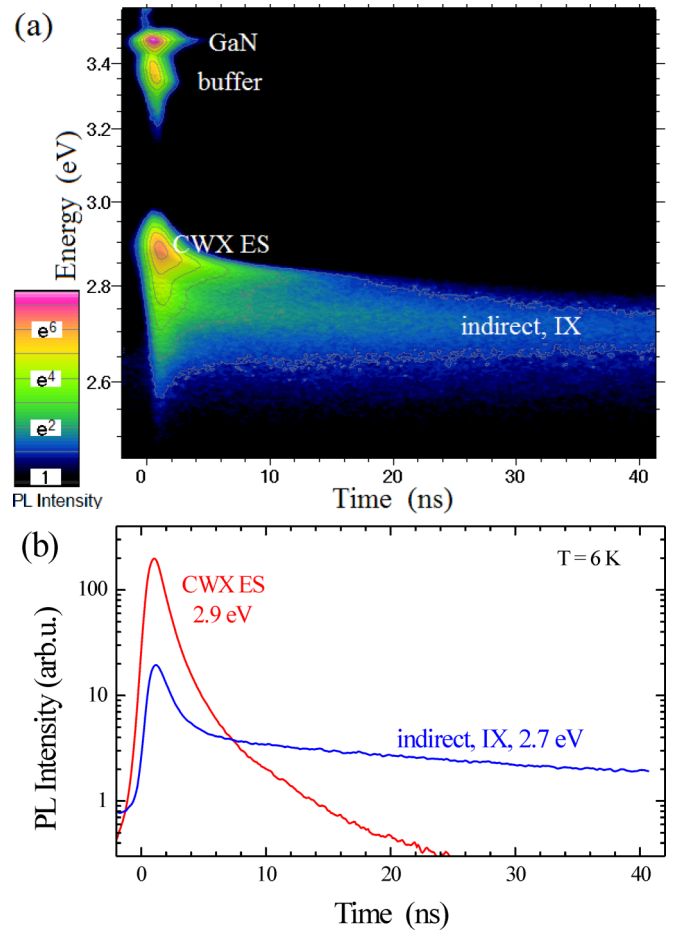
FIG. 9. TRPL of sample C3: (a) full spectrum presented as a contour plot. (b) PL transients observed for CWX-ES and IX (interwell) emissions. The effective power density was 3.5 \text{ kW/cm}^2 .
