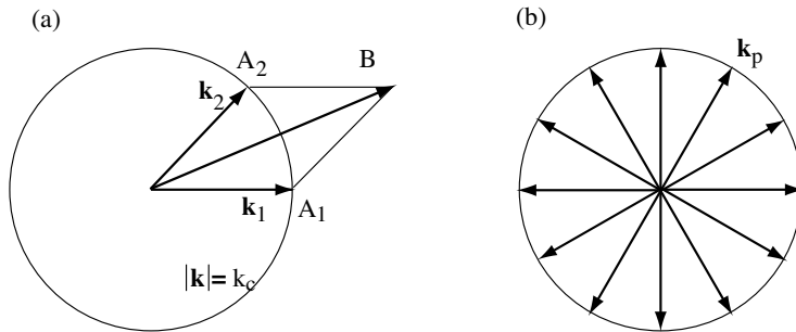
FIGURE 1 – (a) Two neutral modes with wave vectors \mathbf{k}_1 and \mathbf{k}_2 and amplitudes A_1 and A_2 oscillating at \omega/2 , nonlinearly interact to give a wave with wave vector \mathbf{k}_1 + \mathbf{k}_2 and amplitude B oscillating at \omega . In the absence of dissipation, this wave is neutral if \Omega(|\mathbf{k}_1 + \mathbf{k}_2|) = 2\Omega(k_c) = \omega . (b) N neutral modes with wave vectors \mathbf{k}_p at equal angles 2\pi/N on the circle |\mathbf{k}_p| = k_c .
