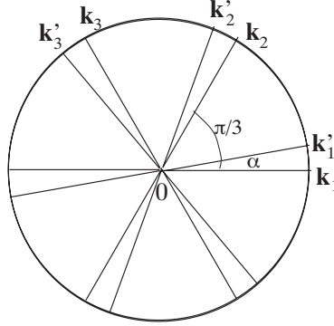
FIGURE 2 – Definition of the lattice \Gamma .
