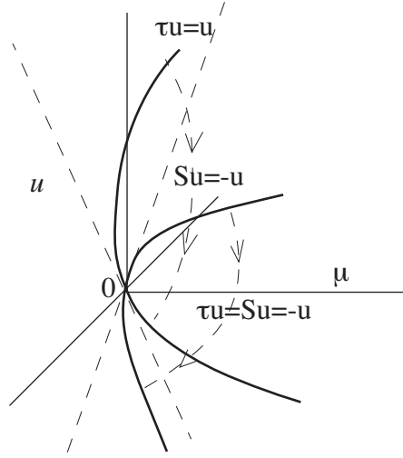
FIGURE 5 – Bifurcating branches of quasipatterns. Actions of symmetries are indicated with arrows.
