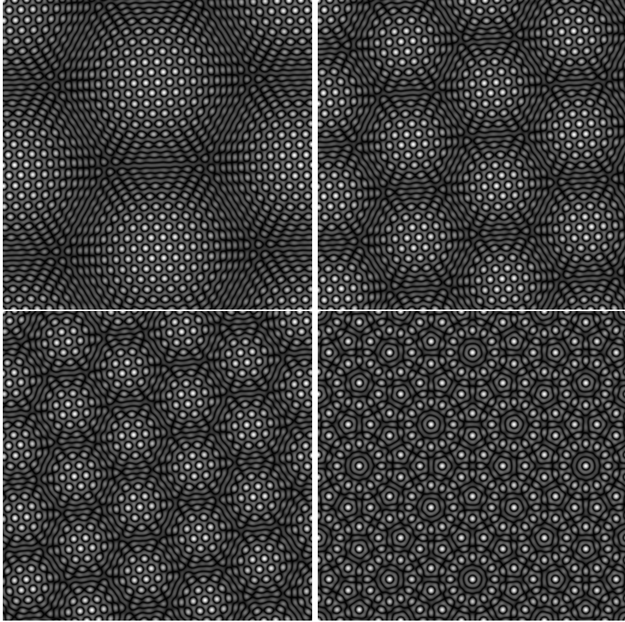
FIGURE 3 – Superposition of two hexagonal patterns for \alpha = 4^\circ, 7^\circ, \pi/18, \pi/6 . Order \varepsilon and \beta_1 = 1 in Theorem 7 is represented.
