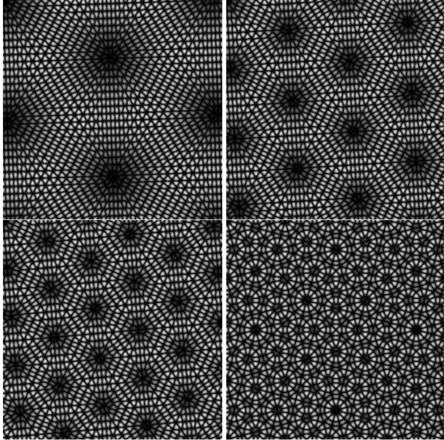
FIGURE 4 – Superposition of two hexagonal patterns for \alpha = 4^\circ, 7^\circ, \pi/18, \pi/6 . Order \varepsilon and \beta_1 = -1 in Theorem 7 is represented.
