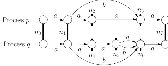
■ Figure 1 A negotiation. Atomic negotiation n_1 involves processes p, q , and has two possible outcomes a and b . The arrows show next negotiations in which respective processes are willing to engage.
