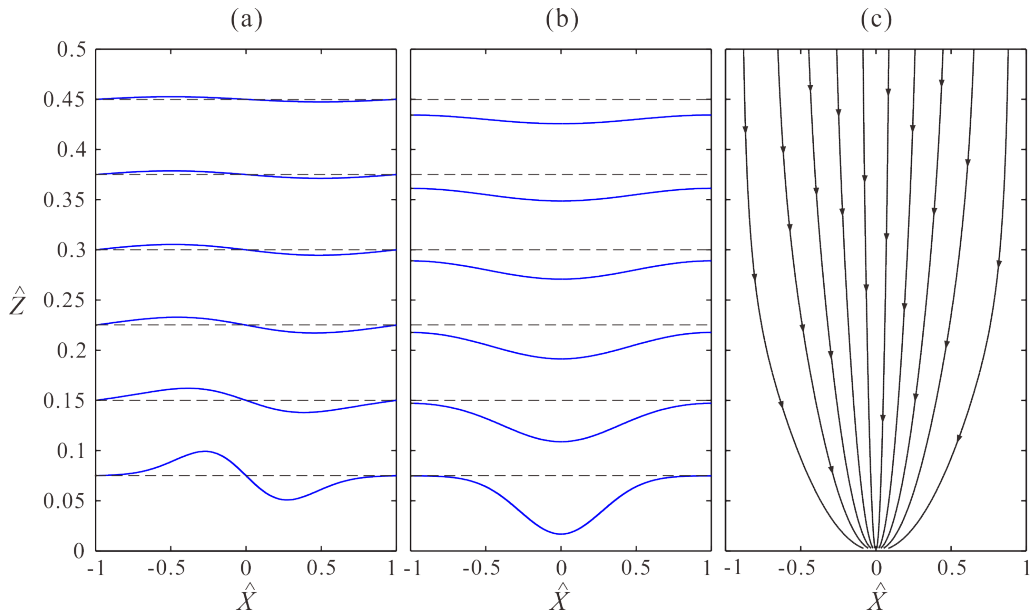
FIGURE 2. Solutions to the kinematic deep flow model: (a) spanwise profiles of horizontal velocity; (b) spanwise profiles of vertical velocity; (c) streamlines.
