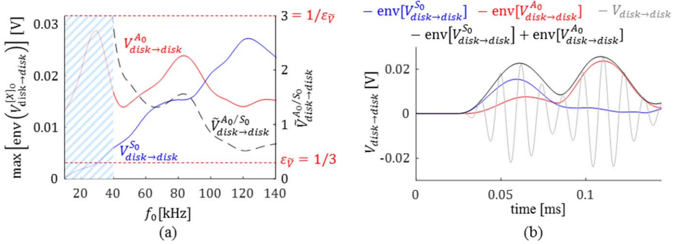
Figure 11. (a) The maximum amplitude of V_{disk \rightarrow disk}^{A_0} and V_{disk \rightarrow disk}^{S_0} in the response signal measured by the disk part of a dual-PZT place for r = 150 mm. The striped area represents the frequency range where the amplitude ratio \tilde{V}_{a \rightarrow s}^{A_0/S_0} (right axis) between the maximum amplitude of V_{disk \rightarrow disk}^{A_0} and V_{disk \rightarrow disk}^{S_0} does not respect the threshold \varepsilon_{\tilde{V}} = 1/3 . (b) The superposition of the contributions of each mode and the signal measured by the disk part of the dual-PZT for f_0 = 80 kHz, at r = 150 mm and \theta = 0^\circ .
