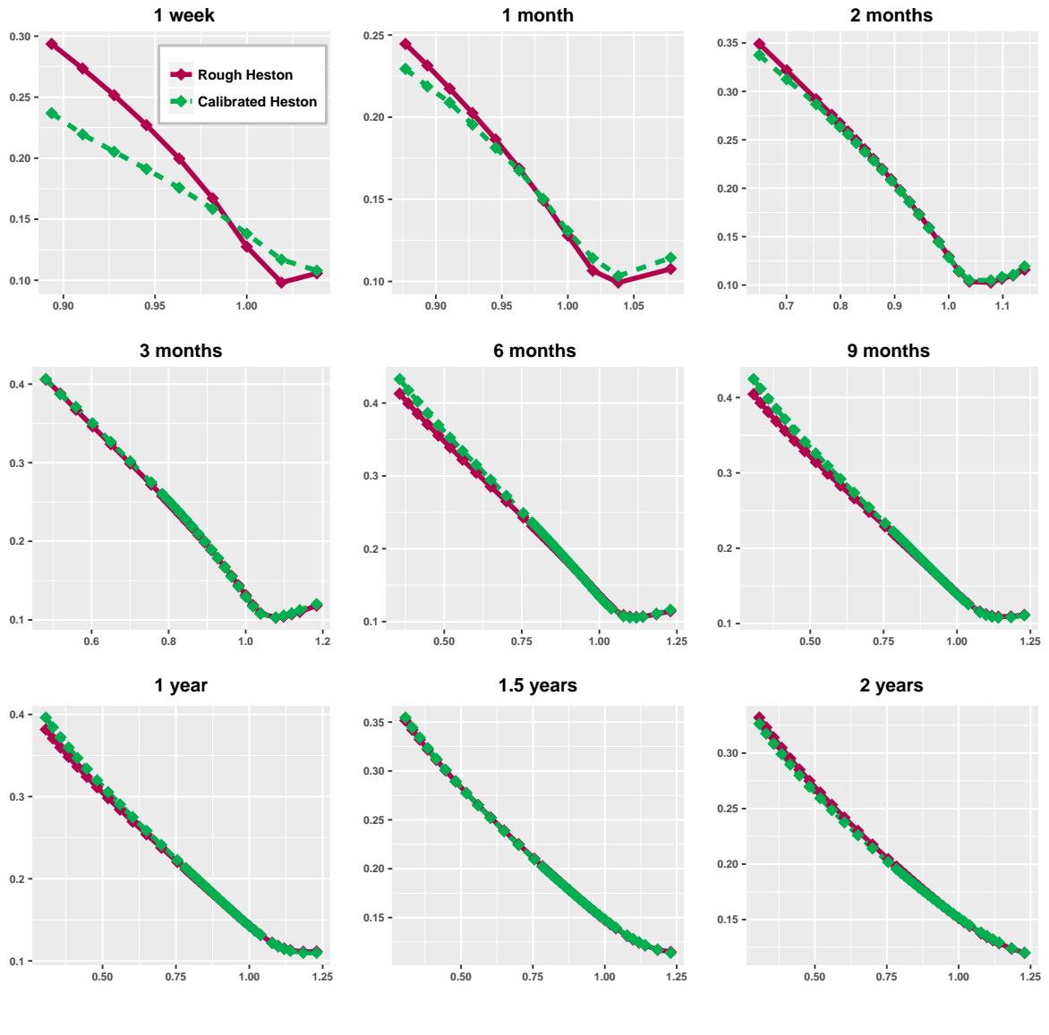
Figure 11: Implied volatility surface of the rough Heston model \sigma_{\infty}(K, T; \Theta_0) (red) and the calibrated Heston model of Table 6 (green) for maturities ranging from 1 week to 2 years (MSE = 2.06e-03).
