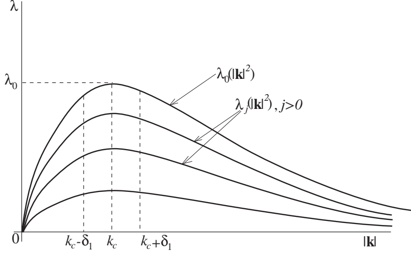
Figure 4: Sketch of positive eigenvalues of \mathcal{A} in function of |\mathbf{k}| , and definition of critical lambda \lambda_0 . \delta_1 is used to define the projection \pi_0 at section 7.4
