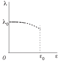
Figure 2: Bifurcation curve. The set of "good" \varepsilon 's is of asymptotically full measure
