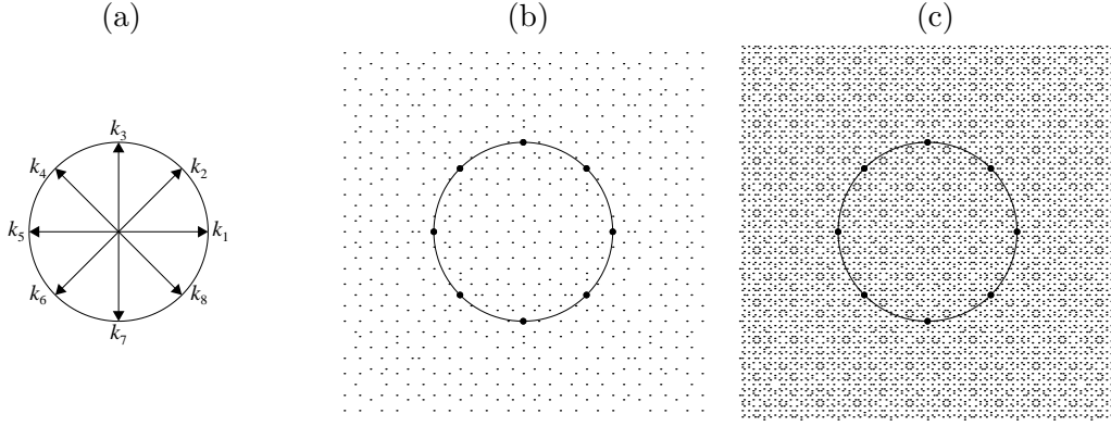
Figure 3: Example of quasilattice with 2q = 8 , after [19]. (a) The 8 wavevectors with |\mathbf{k}| = 1 which form the basis of the quasilattice. (b,c) The truncated quasilattices \Gamma_9 and \Gamma_{27} . The small dots mark the positions of combinations of up to 9 or 27 of the 8 basis vectors on the unit circle.
