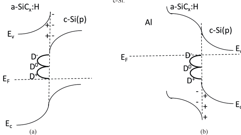
Fig. 7. Evolution of the a-SiC x :H/c-Si band diagram without (a) and with (b) a metallic contact
