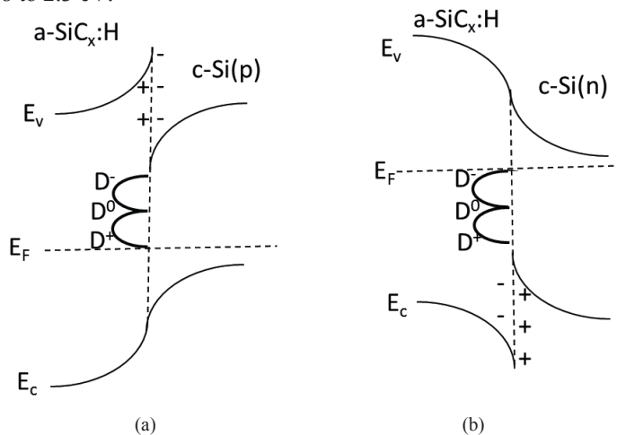
Fig. 6. Band diagram drawing of a-SiC x :H/c-Si interface at equilibrium for p- (a) and n-type (b) silicon (representation of interfacial defects in a-SiC x :H are represented as described for a-Si:H in Olibet et al. [13]). Work function of a-SiC x :H is estimated lower than c-Si.
