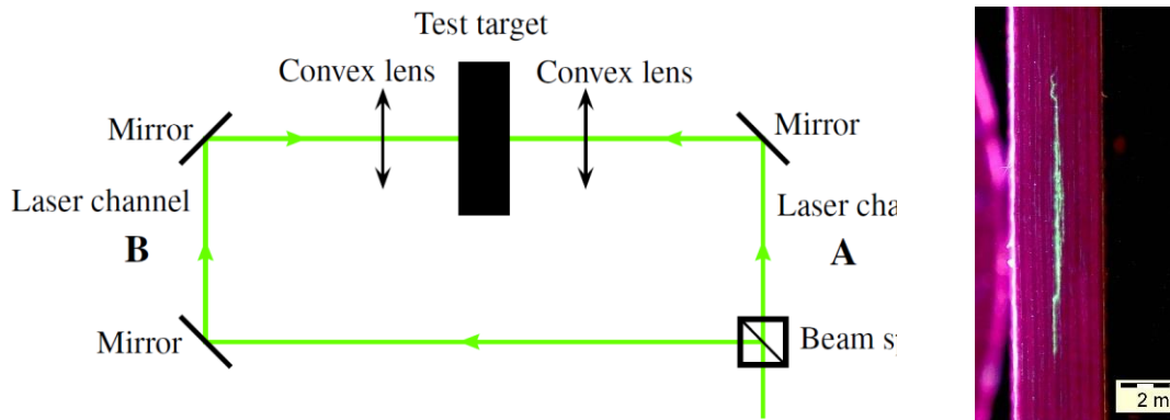
Figure 1: [Left] Experimental set-up of symmetrical laser shock configuration. [Right] Cross-sectional observation showing a delamination generated using LSWT.
