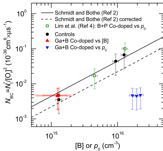
FIG. 2. (Color online) Relative saturated defect density plotted in B-doped controls and in Si co-doped with B and Ga as a function of the B concentration or the carrier density. Solid line is a fit to experimental data on B-doped Si from Ref. 2. Dashed line corresponds to the same fit divided by a correction factor of 2 to account for the defect density reduction expected in P-diffused Si. Open symbols correspond to effective defect density from Ref. 4 measured in P-diffused B and P compensated Si and plotted as a function of p_0 .
