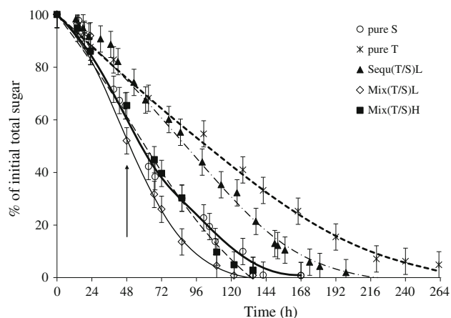
Fig. 1 Residual sugars (in percentage of initial concentration of 220 \text{ g L}^{-1} ) of pure, mixed and sequential cultures of T. delbrueckii and S. cerevisiae in MS300 at 20^\circ \text{C} . “pure S” is pure S. cerevisiae fermentation; “pure T” is pure T. delbrueckii fermentation; “Seq(T/S)L” stands for sequential fermentation with the low ratio; “Mix(T/S)L” for mixed fermentation with the low ratio and “Mix(T/S)H” for mixed fermentation with the high ratio of T/S. The arrow indicates the moment of inoculation of S. cerevisiae in the sequential fermentation
