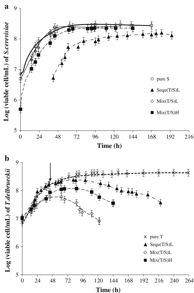
Fig. 2 Cell growth kinetics of viable S. cerevisiae (a) and T. delbrueckii (b) in their pure, mixed and sequential cultures in MS300 at 20^\circ \text{C} . “pure S” stands for pure S. cerevisiae fermentation; “pure T” for pure T. delbrueckii fermentation; “Seq(T/S)L” for sequential fermentation with low ratio; “Mix(T/S)L” for mixed fermentation with low ratio and “Mix(T/S)H” for mixed fermentation with high ratio of T/S, and the arrow indicates the moment of inoculation of S. cerevisiae in the sequential fermentation
