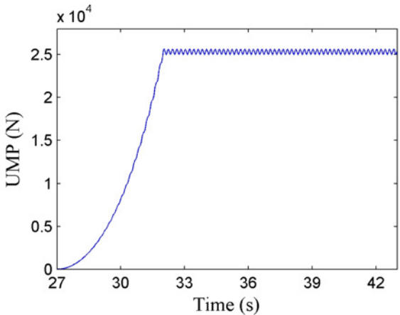
Figure 9. The change of UMP
