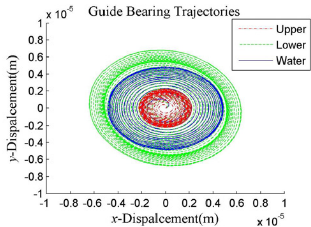
Figure 11. The trajectories of guide bearings' axis
