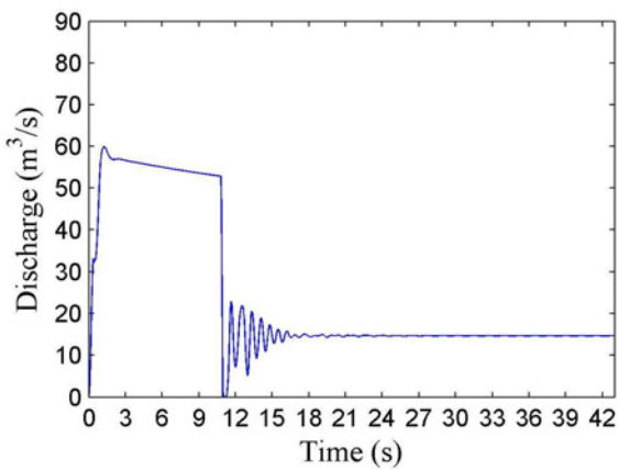
Figure 8. The discharge change during start-up
