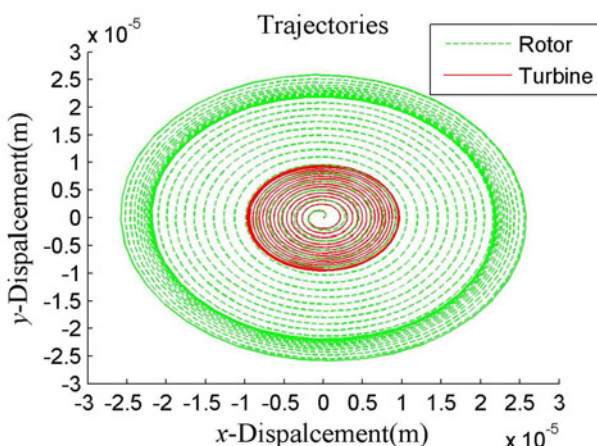
Figure 10. The trajectories of rotators
