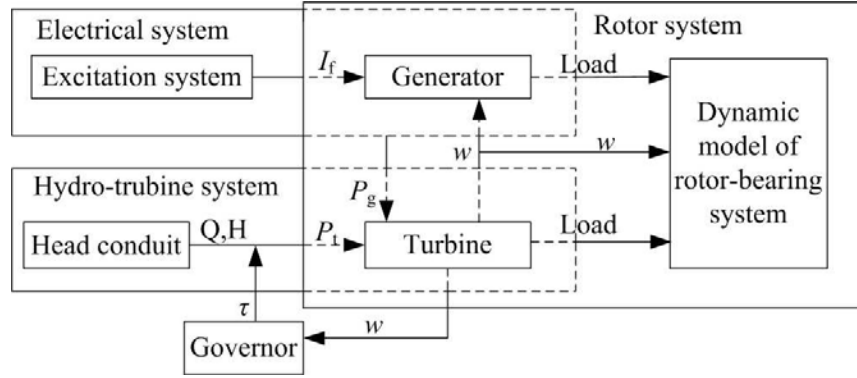
Figure 1. Sketch of Hydropower Plant System
