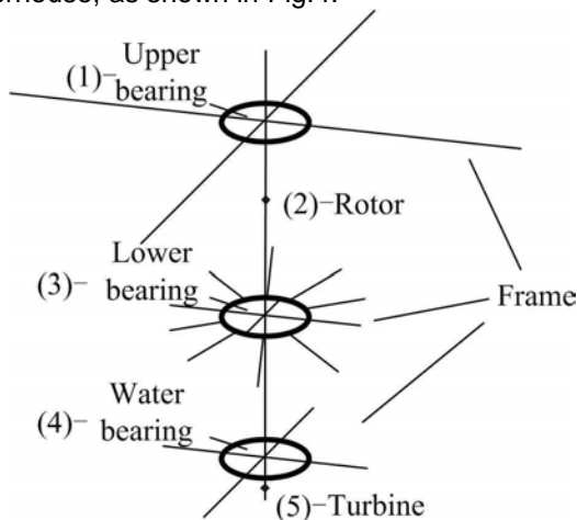
Figure 4. Rotor-bearing model
