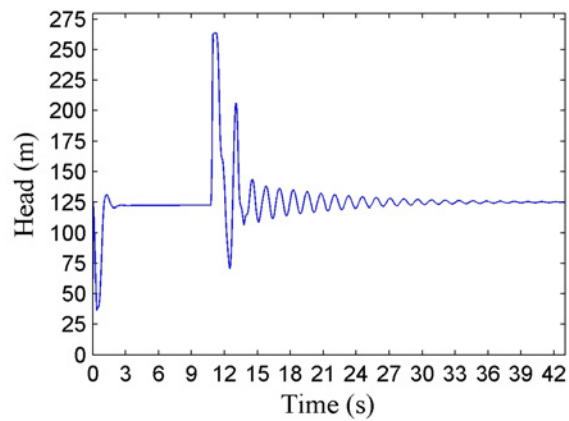
Figure 7. The head change during start-up
