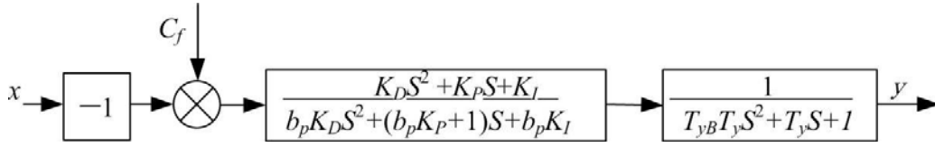
Figure 3. The Transfer Function of the Frequency Regulation Mode
