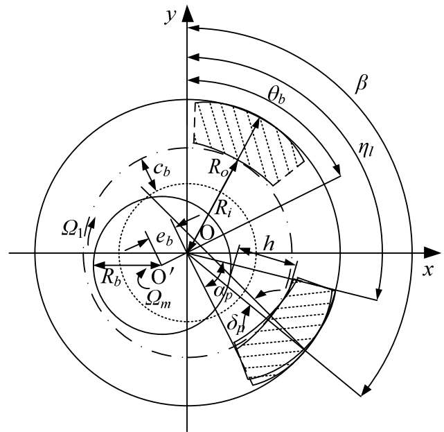
Figure 5. Tilting pad guide bearing
