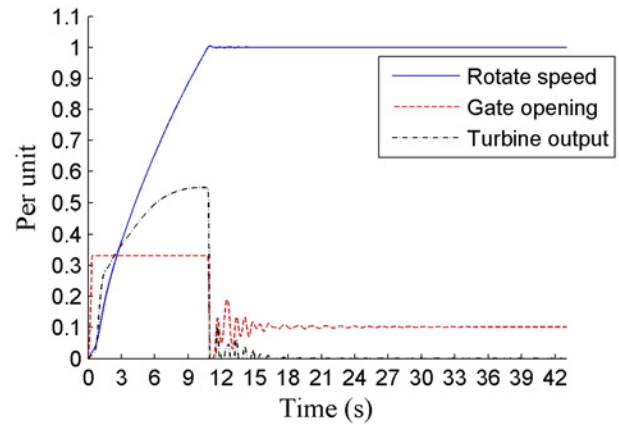
Figure 6. Simulation result of start-up transient
