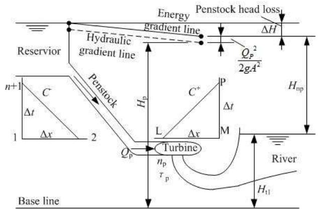
Figure 2. Boundary Condition
