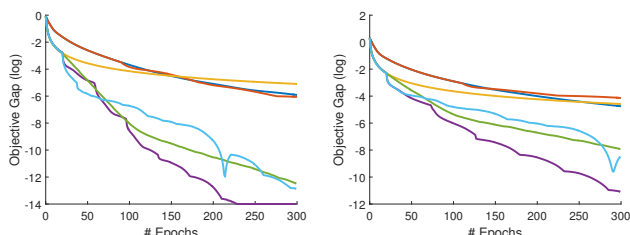
Figure 2: Lasso Regression on Madelon Dataset with 3500 Additional Random Features
