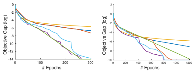
Figure 4: Lasso Regression on the News20 Dataset (Class 1).
