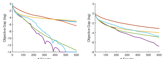
Figure 3: Lasso Regression on MARTI2 Dataset
