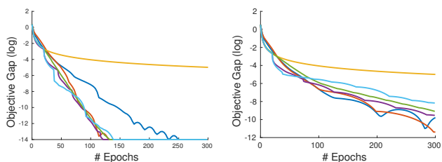
Figure 1: Lasso Regression on RCV1 Dataset
