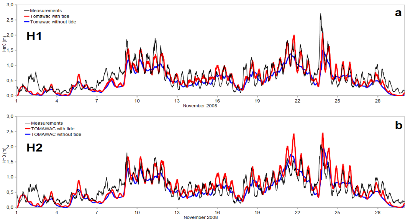
Figure 4. Measured and computed (from experiments E2 and E3) times series of the significant wave height at locations (a) H1 and (b) H2 in November 2008 (from [19]).
