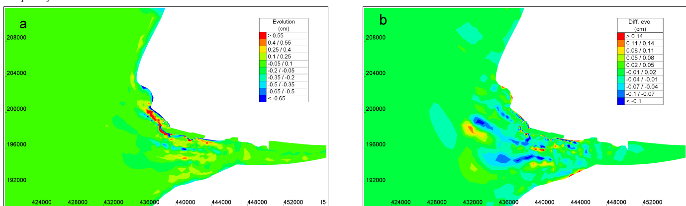
Figure 8. (a) Seabed evolution by suspension of mud at the end of the month of November 2008 for case E3. (b) Differences between the final evolution computed for cases E3 and E2.
