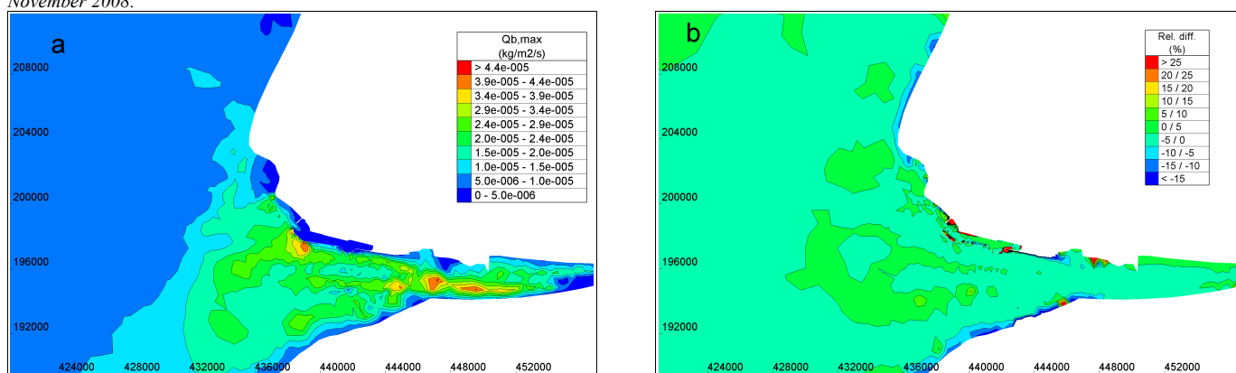
Figure 7. (a) Maximum bedload transport rates of sand for case E3 and (b) relative difference of the maximum bedload transport rates between cases E3 and E2 in November 2008.
