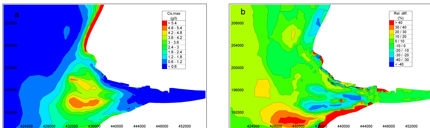
Figure 6. (a) Maximum depth-averaged SSC of mud for case E3 and (b) relative difference of the maximum depth-averaged SSC between cases E3 and E2 in November 2008.
