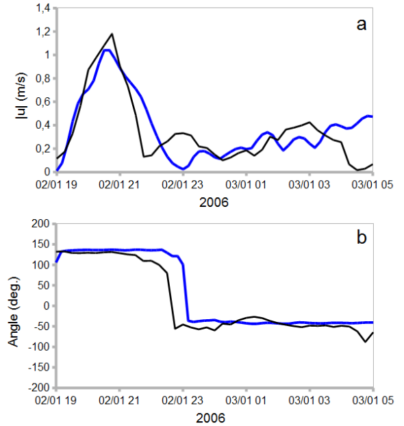
Figure 2. Measured (black) and computed (blue) time series of (a) the module and (b) direction (clockwise from the north) of the depth-averaged currents at location C1 in January 2006 (from [19]).
