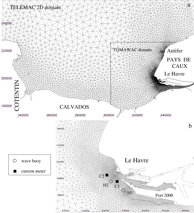
Figure 1. (a) TELEMAC computational domains. (b) Close-up of the computational mesh near the harbour of Le Havre with the locations of the current meters and wave buoys. The coordinates are indicated in meters according to the French system Lambert 1 Nord (from [19]).
