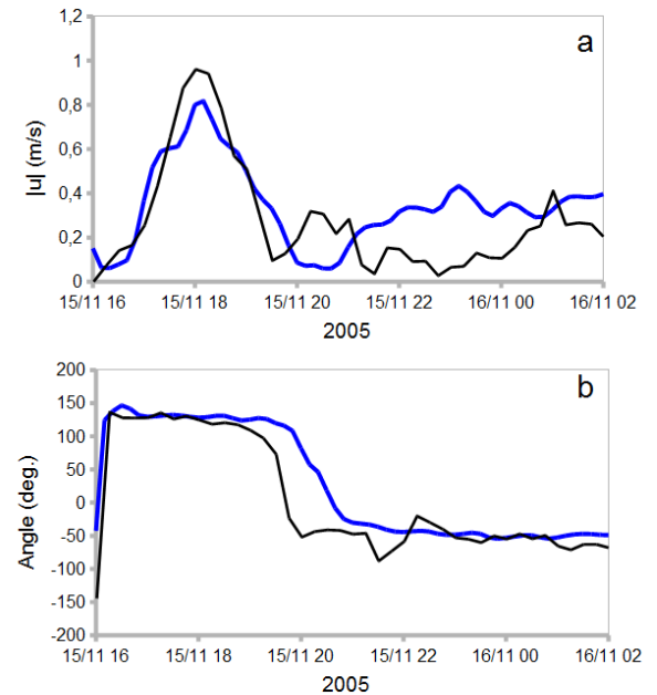
Figure 3. Measured (black) and computed (blue) time series of (a) the module and (b) direction (clockwise from the north) of the depth-averaged currents at location C2 in November 2005 (from [19]).
