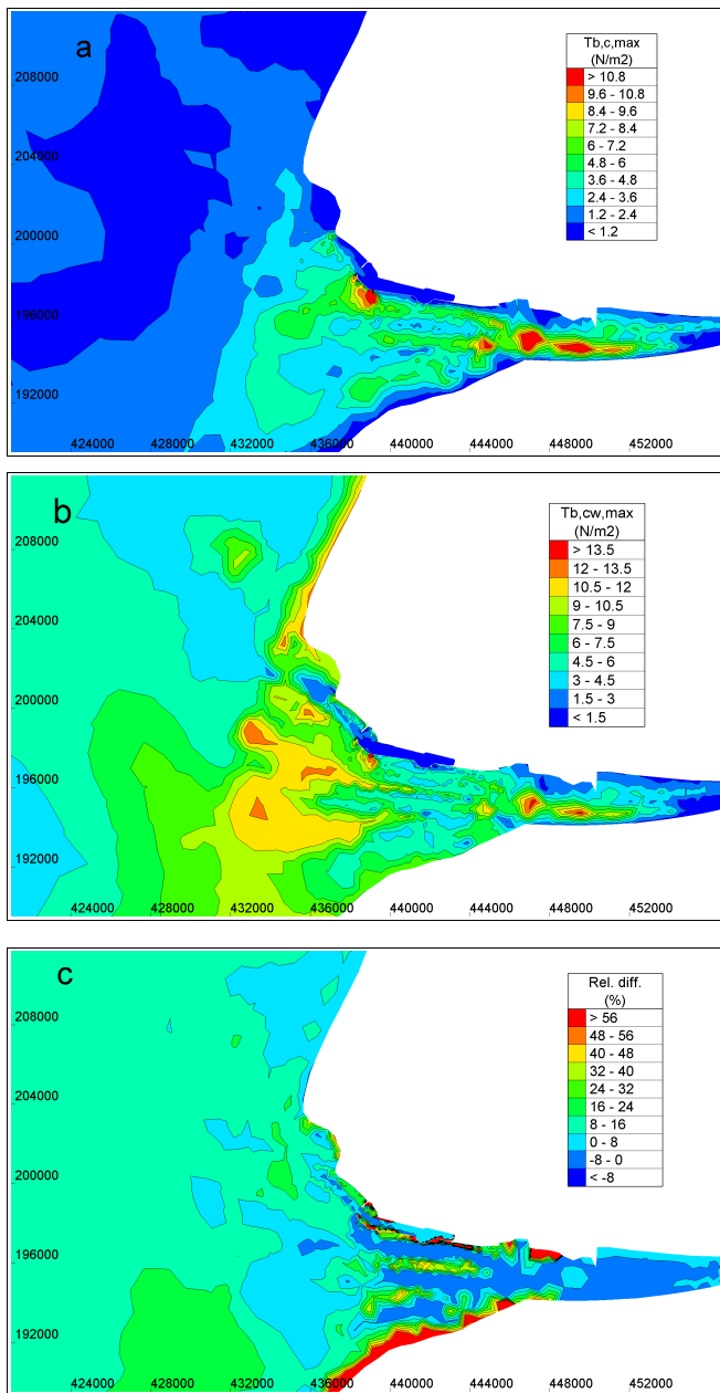
Figure 5. Maximum values of (a) the bottom current shear stress and (b) the total maximum wave and current bottom shear stress for case E3 in November 2008. (c) Relative difference of the maximum value of the total maximum wave and current bottom shear stress in November 2008 between cases E3 and E2.
