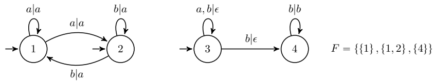
■ Figure 1 Transducer with Muller sets F realizing the function f_{\#a} mapping any word with infinitely many a to a^\omega , otherwise to b^\omega .
