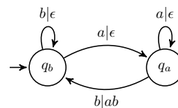
■ Figure 2 Sequential transducer with Muller condition F = \{q_b\} realizing the function f_{ab} which maps any word containing a finite number of a 's to the subsequence of ab factors, and is undefined otherwise.
