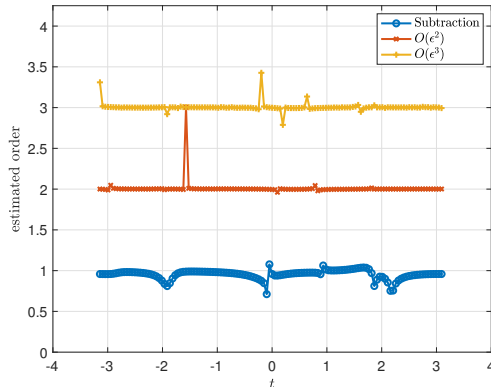
Figure 5: Estimated order of accuracy in computing the double-layer potential in the kite domain when using the subtraction method (blue \circ ), the O(\varepsilon^2) asymptotic approximation method (red \times ), and the O(\varepsilon^3) asymptotic approximation method (yellow + ) for varying values of t .
