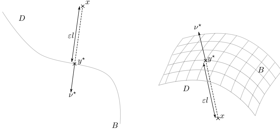
Figure 2: Sketch of the quantities introduced in (2.5) to study evaluation points close to the boundary in 2D (left) and in 3D (right).
