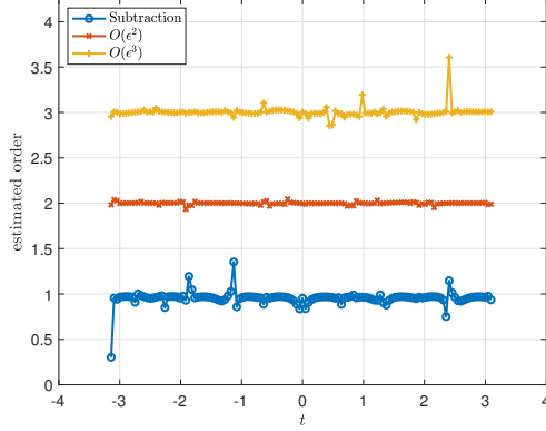
Figure 8: Estimated order of accuracy in computing the double-layer potential in the star domain when using the subtraction method (blue \circ ), the O(\varepsilon^2) asymptotic approximation method (red \times ), and the O(\varepsilon^3) asymptotic approximation method (yellow * ) for varying values of t .
