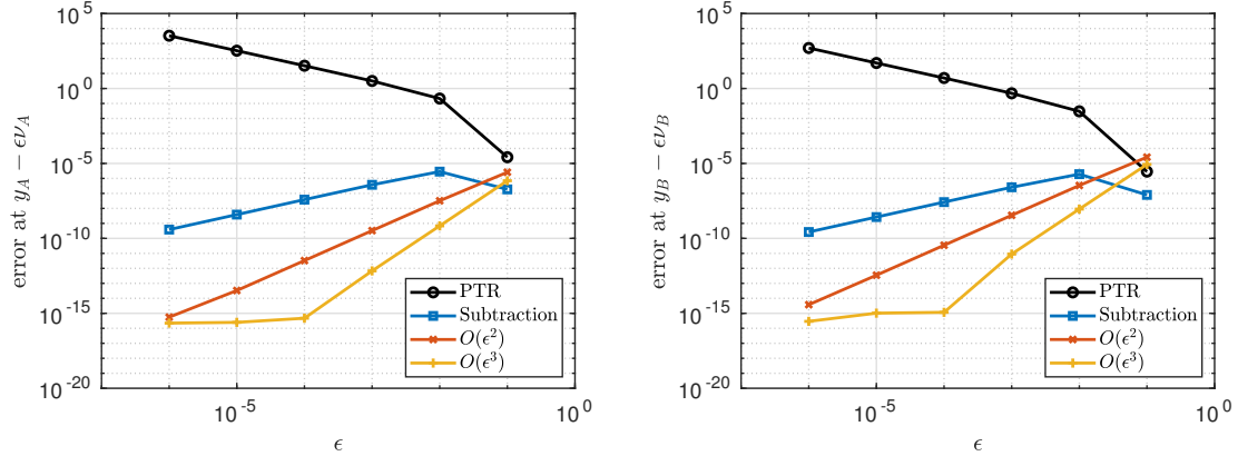
Figure 7: Log-log plots of the errors made in computing the double-layer potential by the four methods shown in Fig. 6 at y_A - \varepsilon\nu_A (left) and at y_B - \varepsilon\nu_B (right) for 10^{-6} \leq \varepsilon \leq 10^{-1} .
