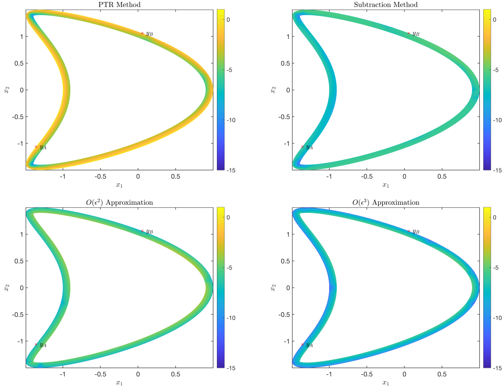
Figure 3: Plots of \log_{10} of the error for the evaluation of the double-layer potential in the kite domain defined by (6.2) using four methods: the PTR method (upper left), the subtraction method (upper right), the O(\varepsilon^2) asymptotic approximation method (lower left), and the O(\varepsilon^3) asymptotic approximation method (lower right). In each of these plots, boundary points y_A = (-1.3571, -1.0607) and y_B = (0.0571, 1.0607) are plotted as red \times 's.
