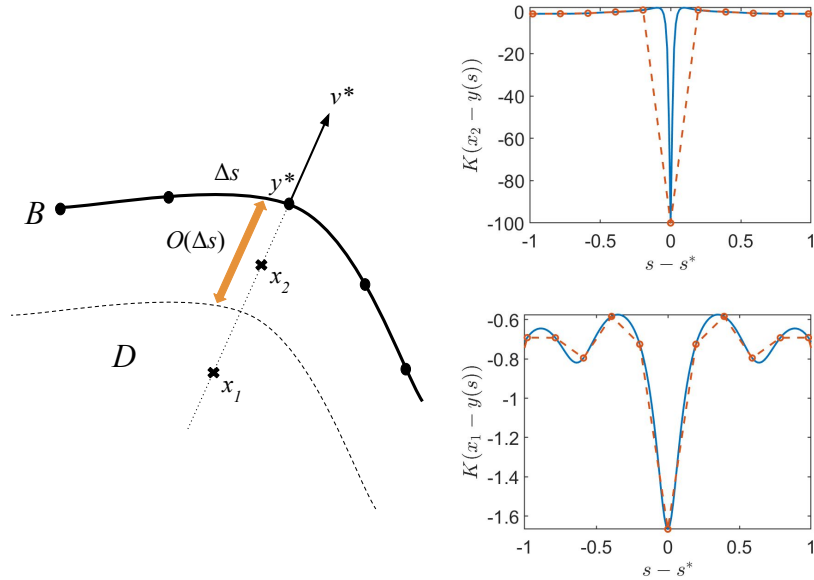
Figure 1: 2D sketch showing the finite length scale, \Delta s , of the discretization for (2.1) which leads to the close evaluation problem. For the point x_1 which is farther than \Delta s from the boundary, we find that the kernel is well resolved with the boundary grid. However, for the same boundary grid, we find that the kernel is poorly resolved for x_2 , which is closer to the boundary than \Delta s . In each plot on the right, the kernel K(x_i - y(s)) := \frac{\nu_y \cdot (x_i - y(s))}{|x_i - y(s)|^2} , i = 1, 2 , is plotted in blue, and a piece-wise linear approximation using a fixed \Delta s grid is plotted in dashed orange.
