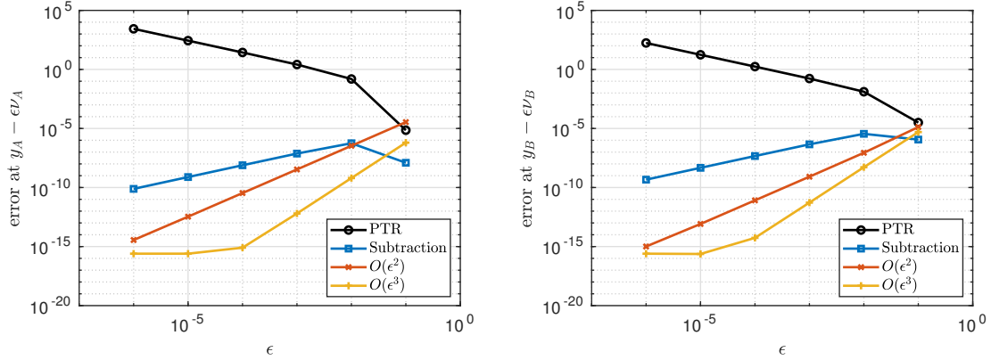
Figure 4: Log-log plots of the errors made in computing the double-layer potential by the four methods shown in Fig. 3 at y_A - \varepsilon\nu_A (left) and at y_B - \varepsilon\nu_B (right) for 10^{-6} \leq \varepsilon \leq 10^{-1} .
