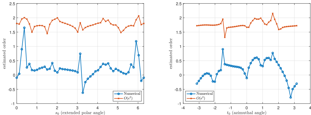
Figure 12: Estimated order of accuracy for the numerical approximation (blue \circ ), and the O(\varepsilon^2) asymptotic approximation (red \times ) on the x_1x_3 -plane (left plot) and on the x_1x_2 -plane (right plot). Results on the x_1x_3 -plane are given in terms of the extended polar angle, s_0 \in [0, 2\pi] , which parameterizes the circle on the unit sphere lying on the x_1x_3 -plane that starts and ends at the north pole. Results on the x_1x_2 -plane are given in terms of the azimuthal angle, t_0 \in [0, 2\pi] .
