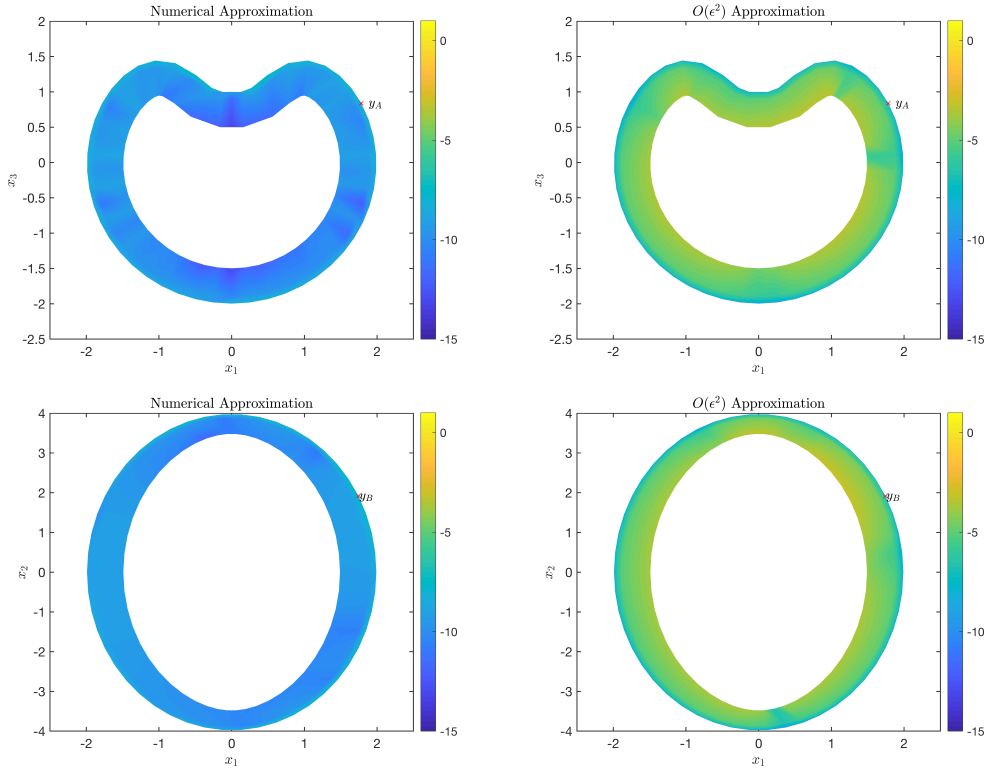
Figure 10: Plots of \log_{10} of the error made in computing the double-layer potential by the numerical approximation (left column) and the O(\varepsilon^2) asymptotic approximation (right column) in the domain whose boundary is shown in Fig. 9. The top row of plots show the error on the x_1x_3 -plane, and the bottom row of plots show the error on the x_1x_2 -plane. In the top row of plots, the point y_A = (1.7830, 0, 0.8390) is plotted as a red \times , and in the bottom row of plots, the point y_B = (1.7439, 1.19175, 0) is plotted as a red \times .
