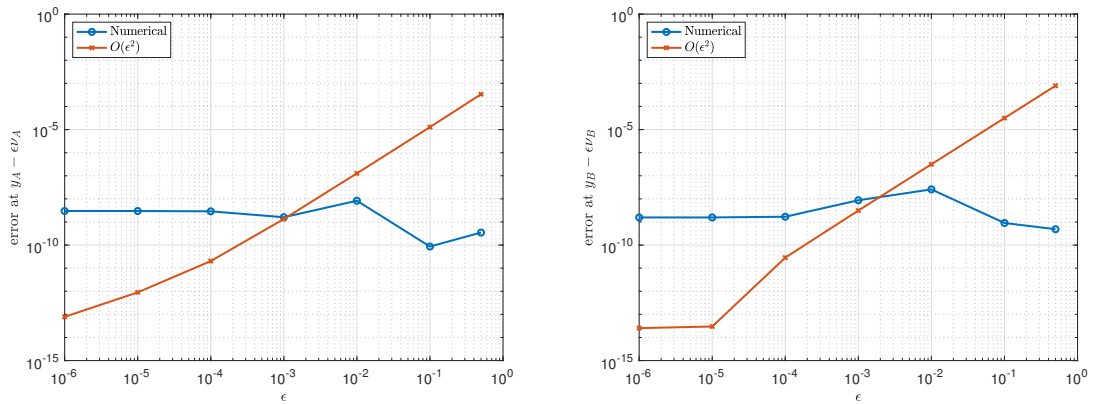
Figure 11: Log-log plots of the errors made by the two methods shown in Fig. 10 at y_A - \varepsilon\nu_A (left) and at y_B - \varepsilon\nu_B (right) for 10^{-6} \leq \varepsilon \leq 0.5 .
