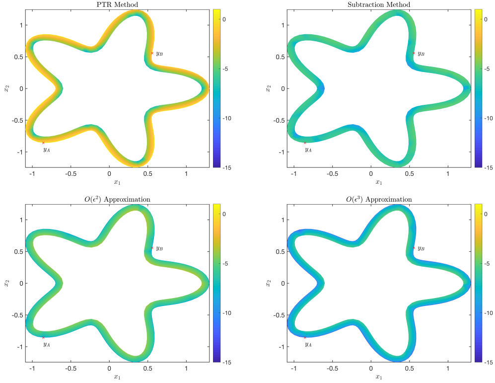
Figure 6: Plots of \log_{10} of the error for the evaluation of the double-layer potential in the star domain defined by (6.3) using four methods: the PTR method (upper left), the subtraction method (upper right), the O(\varepsilon^2) asymptotic approximation method (lower left), and the O(\varepsilon^3) asymptotic approximation method (lower right). In each of these plots, boundary points y_A = (-1.3571, -1.0607) and y_B = (0.0571, 1.0607) are plotted as red \times 's.
