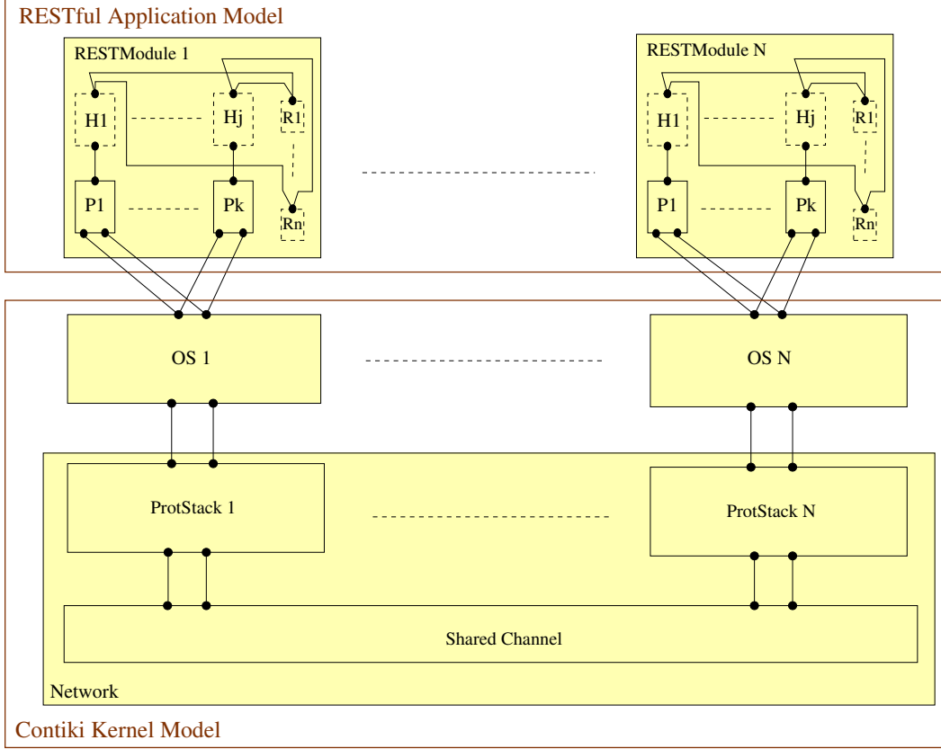
Figure 6: BIP model structure for Contiki WPAN systems
