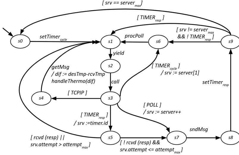
Figure 13: Client process of the building automation application
