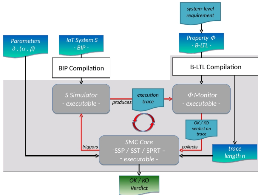
Figure 3: Architecture of the SMC-BIP tool for statistical model checking (source: SMC-BIP website 1 )
