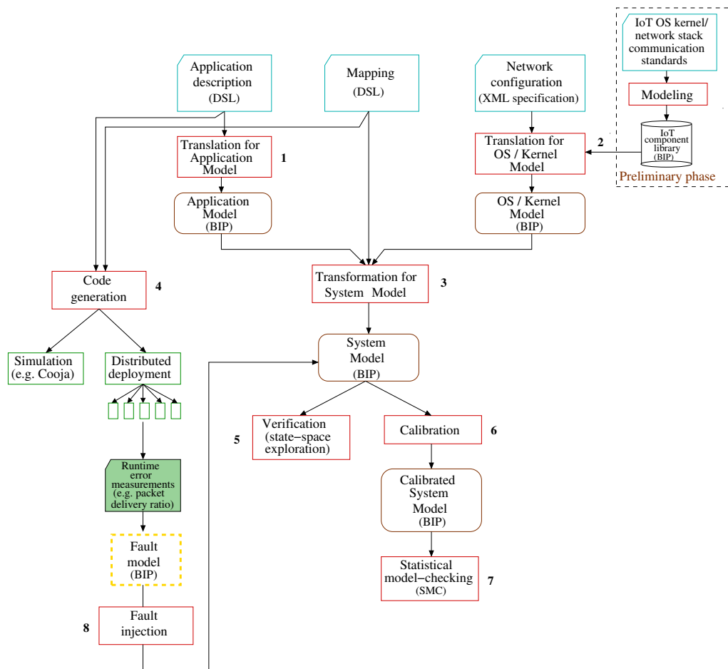
Figure 4: The BIP model-based design flow for IoT WPAN systems (numbered rectangles show the process steps)
