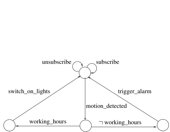
Figure 11: State flow for motion detection by the zone-controller (alarm triggered in non-office hours)
