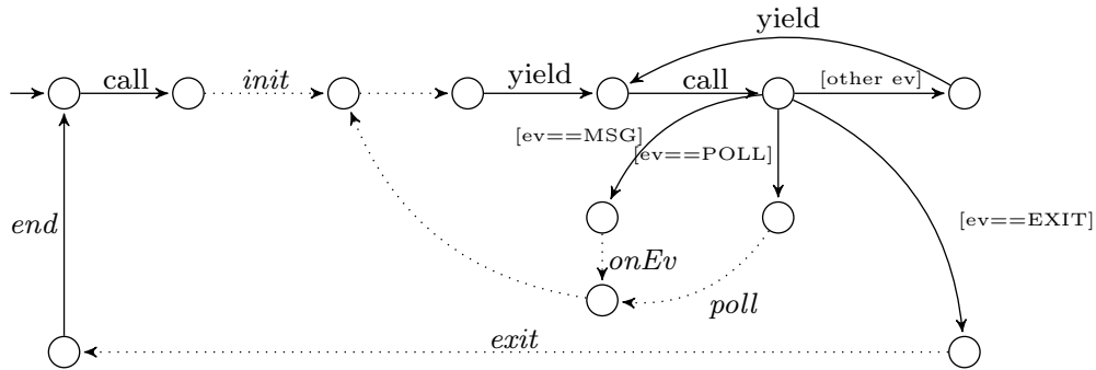
Figure 5: BIP template for the client (all event handlers of Listing 2 are composed in a single automaton)
