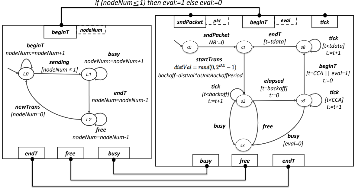
Figure 2: Example BIP components and their interactions - Channel (left) and ProtStack.MsgSender (right)
