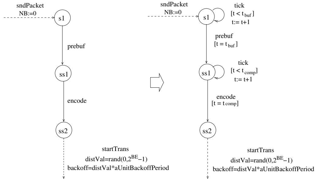
Figure 7: New transitions/guards for the calibration of the \text{ProtStack.MsgSender} component of Figure 2
