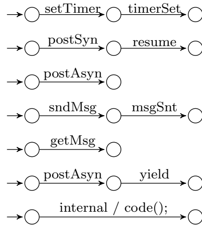
Figure 17: BIP templates for actions in Listing 6
