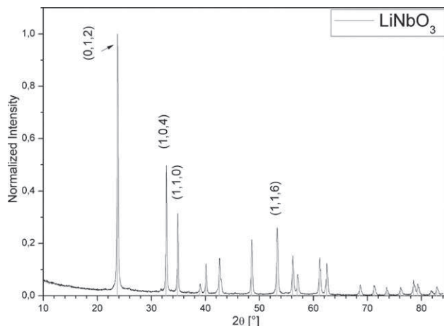
Figure 1. X-ray diffraction pattern of LiNbO 3 nanoparticles.
