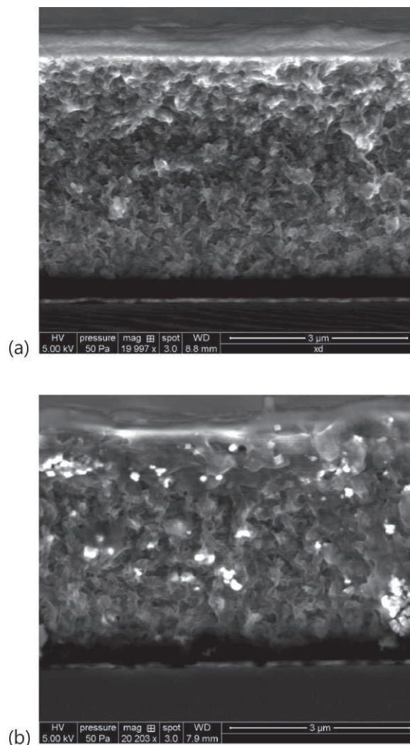
Figure 4. ESEM images of (a) P(VDF-TrFE) and (b) P(VDF-TrFE)/LiNbO 3 10 wt %.
