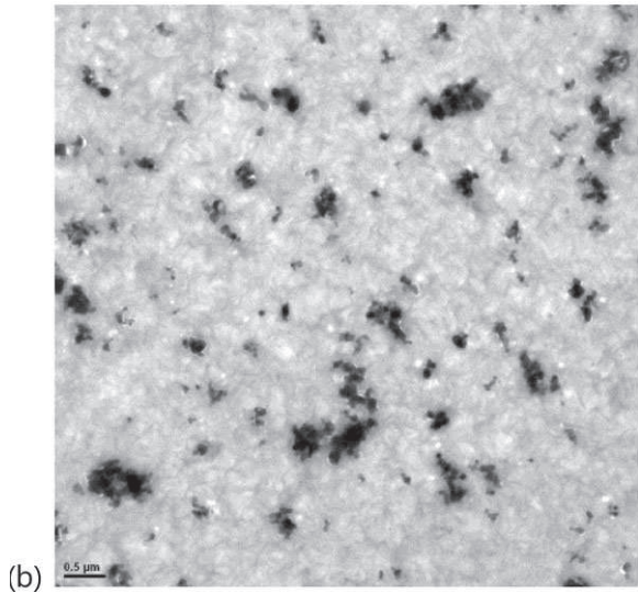
Figure 5. TEM micrographs of (a) P(VDF-TrFE) and (b) P(VDF-TrFE)/LiNbO 3 10 wt %.
