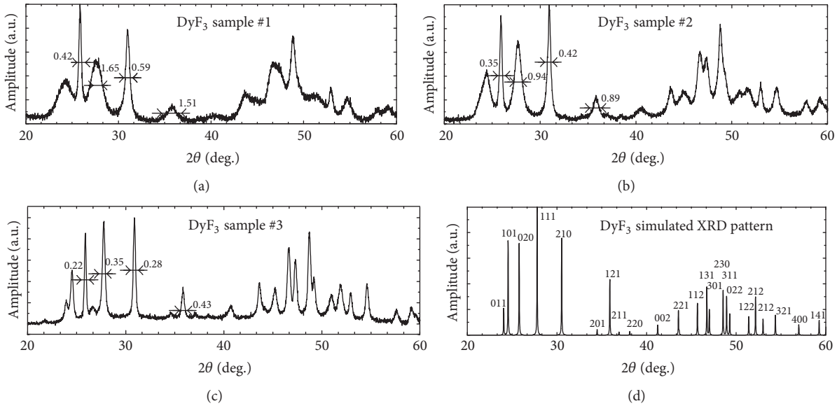
FIGURE 2: (a)–(c) Experimental XRD patterns of synthesized \text{DyF}_3 nanosized samples #1–3. (d) simulated XRD patterns in PowderCell software.
