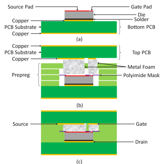
Fig. 1. Embedding of a MOSFET using pressed metal foam. (a): the die is soldered on the bottom PCB; (b): prepreg layers, a polyimide mask & pieces of metal foam (one for each top-side pad) are positioned; (c): the stack is laminated, the epoxy resin polymerizes and floods the foam.
