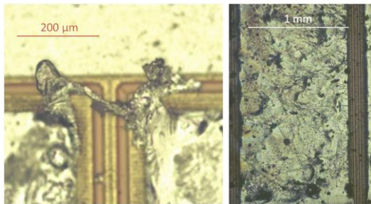
Fig. 14. Melted aluminium above the passivation protecting a gate finger (the dendrite of aluminium is roughly 25 \mu\text{m} -high; left image) and below the piece of foam (right image).
