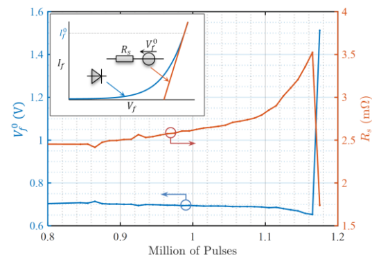
Fig. 7. Inset: measured characteristic (blue) and model (red) of a diode, for a given current I_f^0 . Main plot: evolution of the resistance R_s and voltage source V_f^0 modeling a diode packaged using our process until failure – aging by current surges. I_f^0 = 20 A.
