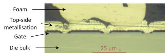
Fig. 4. Cross-sectional view of a contact between the foam and the die.
