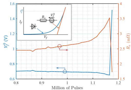
Fig. 7. Inset: measured characteristic (blue) and model (red) of a diode, for a given current I_f^0 . Main plot: evolution of the resistance R_s and voltage source V_f^0 modeling a diode packaged using our process until failure – aging by current surges. I_f^0 = 20 A.
