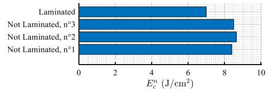
Fig. 12. Energy density leading to failure of CPM2-1200-0025b dies.
