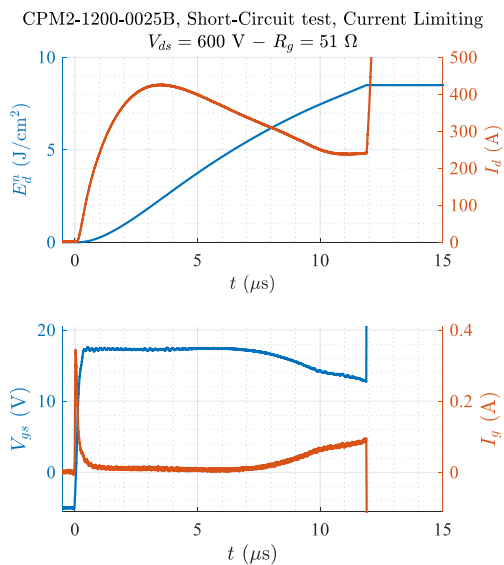
Fig. 11. Waveforms acquired during the tests on a sample: drain current and cumulative dissipated energy (top); gate to source voltage and gate current (bottom).
