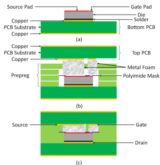
Fig. 1. Embedding of a MOSFET using pressed metal foam. (a): the die is soldered on the bottom PCB; (b): prepreg layers, a polyimide mask & pieces of metal foam (one for each top-side pad) are positioned; (c): the stack is laminated, the epoxy resin polymerizes and floods the foam.
