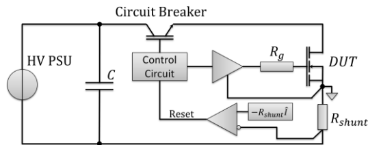
Fig. 9. Schematic of the set-up used in current-limiting tests.
