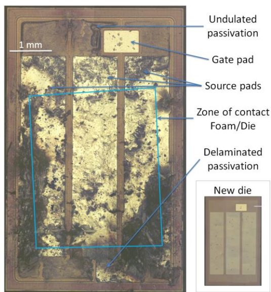
Fig. 13. Photography of a die before and after test.
