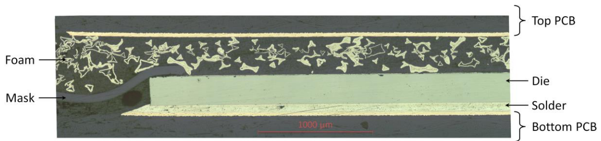
Fig. 2. Partial cross-sectional view of an embedded diode. The die is 250 µm-thick and 6.5 mm-wide.
