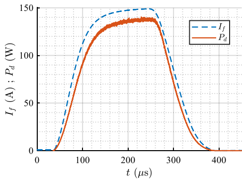
Fig. 5. Current and dissipated power during a current surge.
