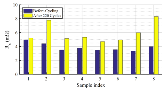
Fig. 8. Resistance of diodes packaged using our process before and after thermal cycling; I_f^0 = 10 \text{ A}
