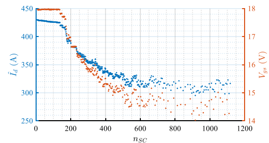
Fig. 15. Peak saturation current (blue) and on-state gate to source voltage (red) vs. number of short-circuits
