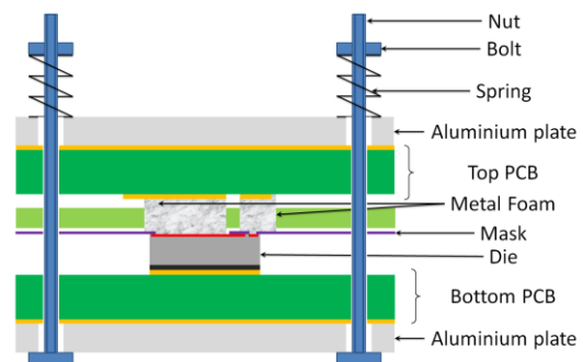
Fig. 10. Schematic of the press-pack-like mechanical set-up used for the tests.
