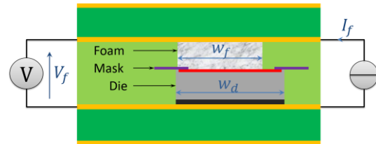
Fig. 6. Kelvin-connection of an embedded diode to the curve tracer: current source and voltage sensing, connected on the right- and left- hand side in the schematic, respectively.
