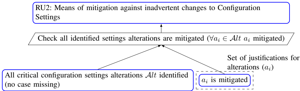
Fig. 3. JP-RU2: Means of mitigation against inadvertent changes to Critical Configuration Settings.
