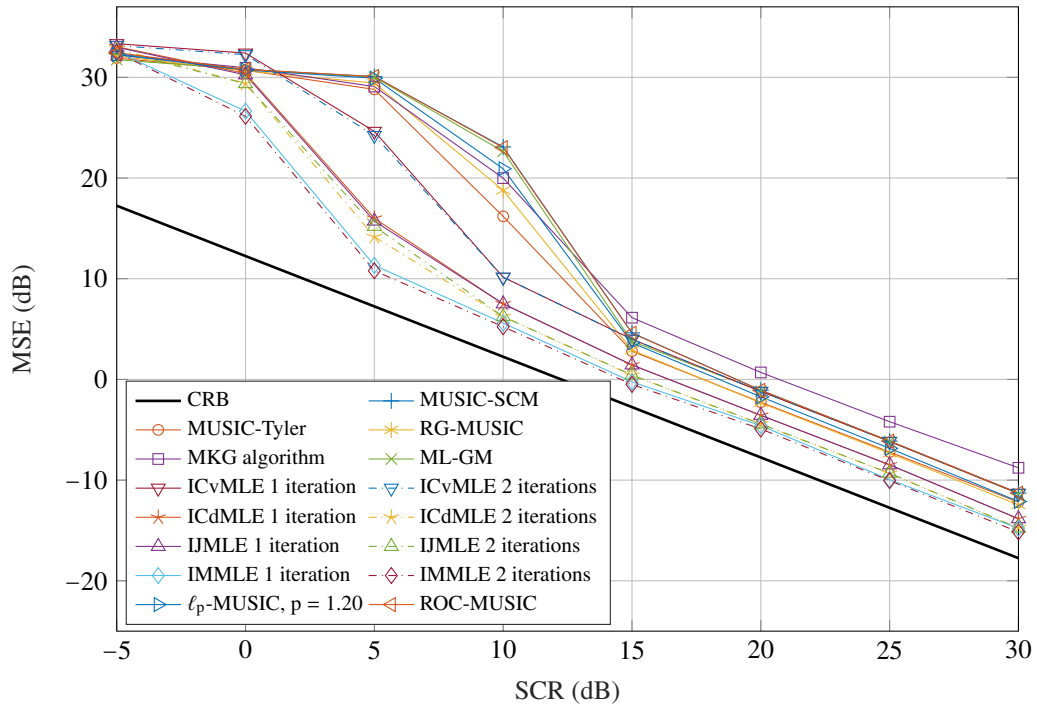
Figure 1: MSE vs. SCR under K-distributed clutter, L = 15
