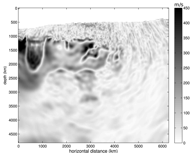
Figure A7. BP case study without noise. Standard deviation (in \text{m s}^{-1} ) of the final velocity model over 50 realizations using source encoding associated to model shown in Fig. A6(d).
