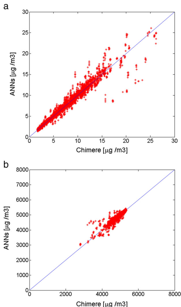
Fig. 2. Surrogate model validation scatter plots, for (a) yearly \text{NO}_2 and (b) summer \text{SOMO35} indicators. The value simulated by the CHIMERE deterministic model is on the horizontal axis, and that obtained with the ANN surrogate model is on the vertical axis.
