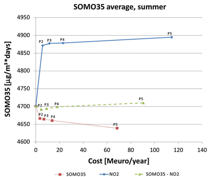
Fig. 5. Pareto optimal policies computed considering the three selected optimizations, with cost of policy implementation (horizontal axis) and SOMO35 summer values (vertical axis). The blue line corresponds to the NO_2 optimization, the red dotted line to the SOMO35 optimization, and the green dashed line to the multi-pollutant case.
