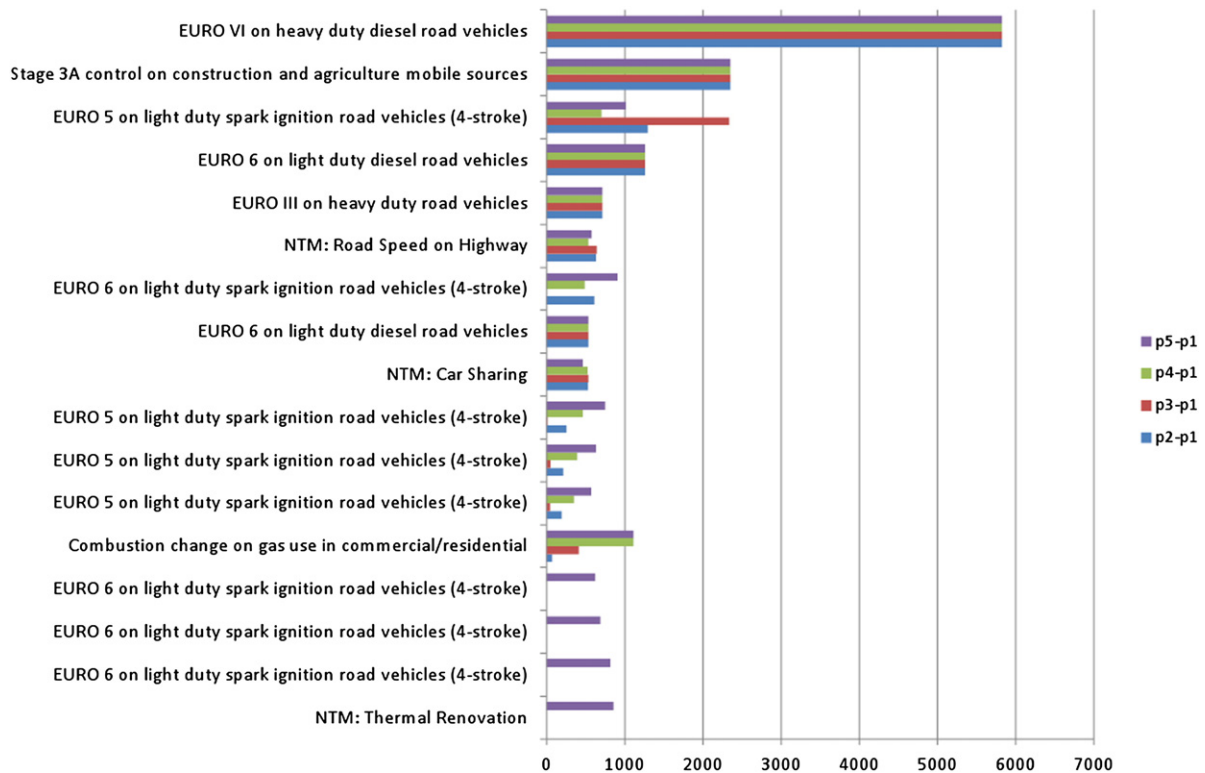
Fig. 7. Main NO_x emission reduction measures, in the case of NO_2 optimization, for different points of the Pareto curve. Bars are related to the reductions beyond CLE (i.e. point P1) for the different points from P2 to P5 (i.e. P3–P1 represent the emission reduction needed to move from CLE to the third point of the curve).
