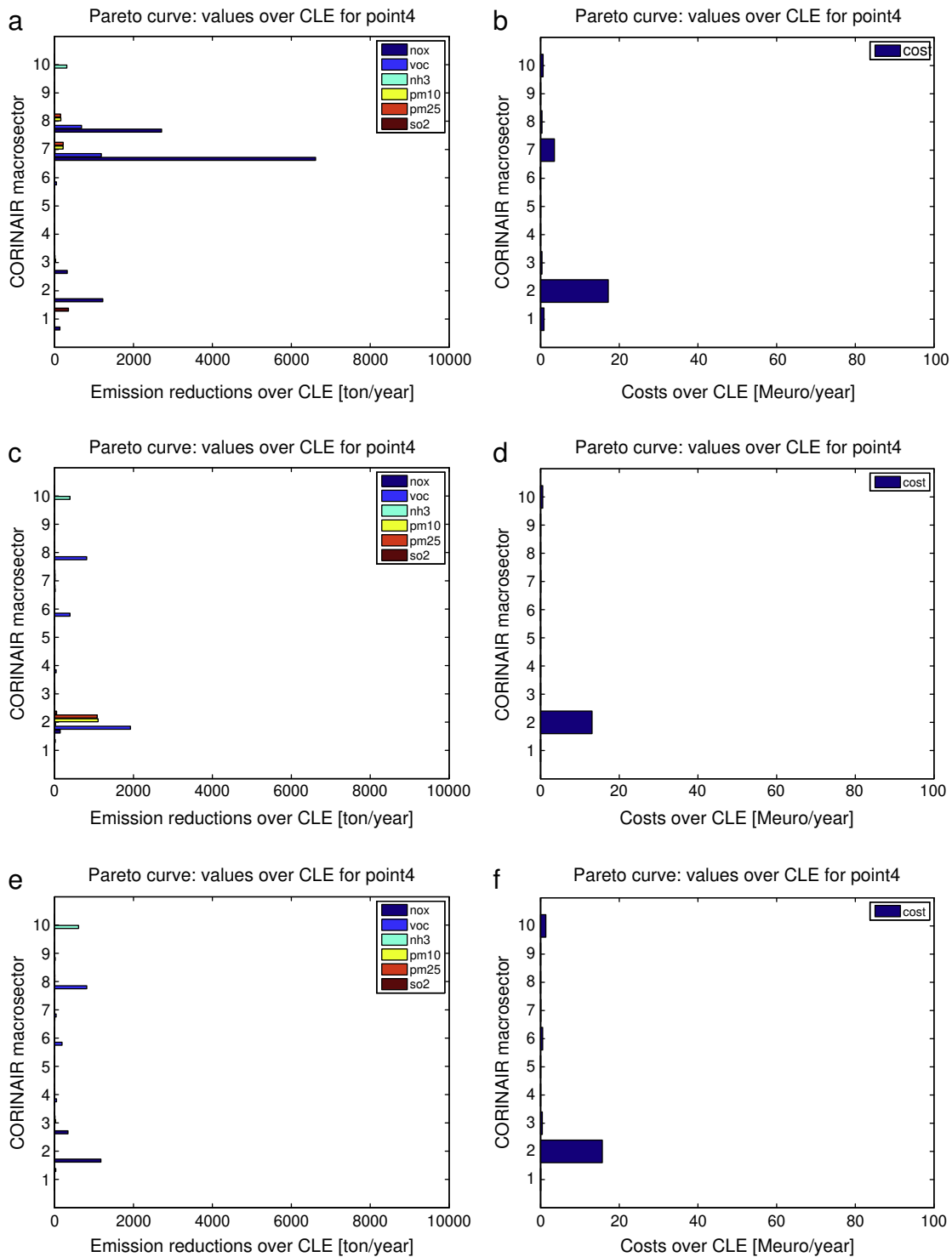
Fig. 6. Emission reductions (left column) and costs (right column) beyond CLE, corresponding to the optimal policies computed for point P4 of the Pareto curve, for (a, b) yearly NO_2 optimization; (c, d) summer SOMO35 optimization; (e, f) joint NO_2 and SOMO35 optimization.
