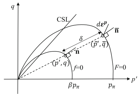
Fig. 4 Bounding surface, Loading surface, and the radial mapping method
