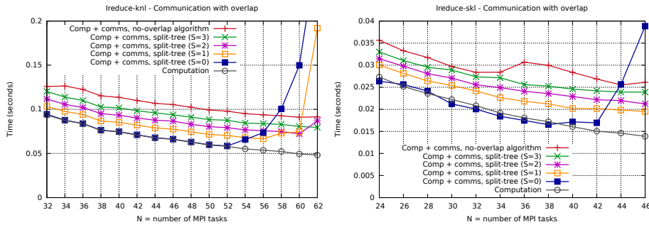
Fig. 6. Result of split-tree algorithm with different values of S, for MPI.Ireduce with constant-size buffer of 2MB on KNL (left) and Skylake (right) processors.
