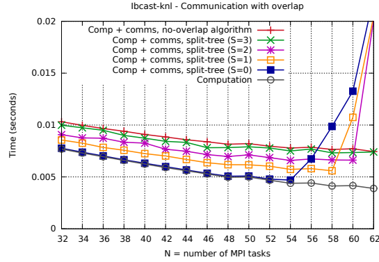
Fig. 5. Result of split-tree algorithm with different values of S, for MPI.Ibcast with constant-size buffer of 2MB on 64 cores (KNL).
