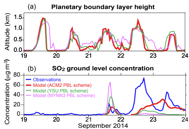
Figure 13. Time variations in Lille of modelled (top) planetary boundary layer height and (bottom) SO 2 concentration at ground-level with high spatial resolution simulations configured with YSU (green), ACM2 (red) and MYNN3 (pink) PBL parameterization schemes. The observed ground-level concentration is represented in blue.
