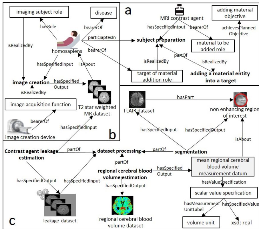
Fig. 3 Representation of the mean rCBV measurement process with the IBO ontology: box a describes the entities that are involved in the subject preparation process, box b corresponds to the image creation process, box c details the dataset processing processes. We note that processes are represented in bold , classes that are not processes are contained in boxes and relationships are denoted with arcs.
