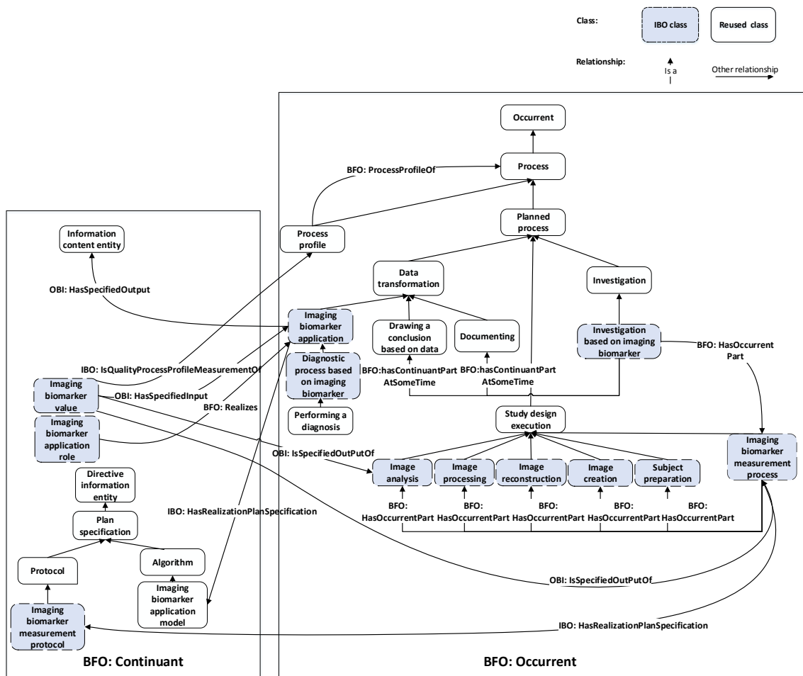
Fig. 2 An extract illustrating the core structure of the BFO:occurrent part defining the IBO ontology. Boxes represent classes (blue ones refer to main concepts of semantic axis), and arcs refer to relationships between them: axioms and subsumption relationships. The subsumption “is a” relationship is denoted by unlabeled arcs.
