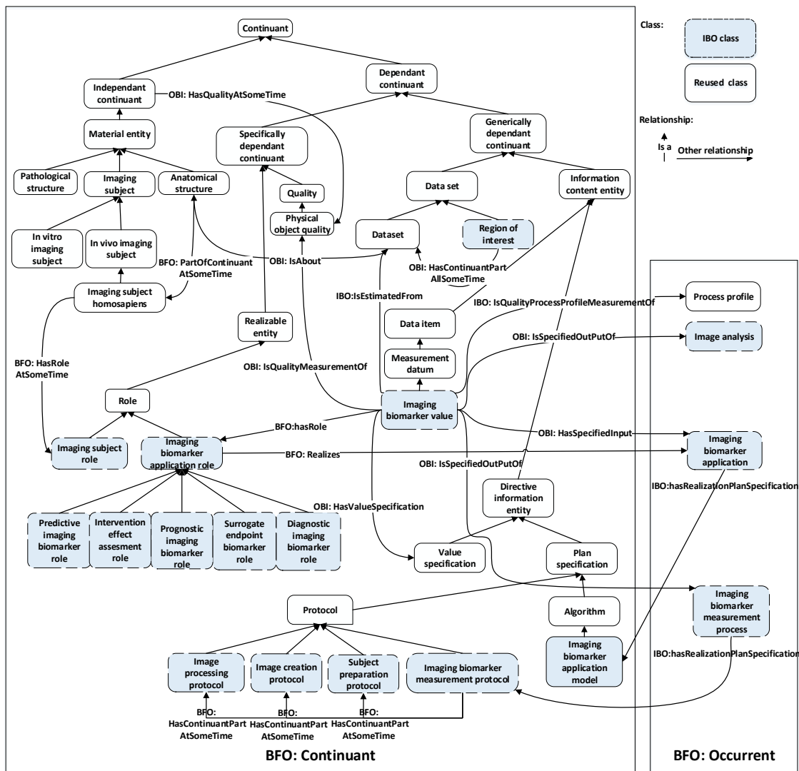
Fig. 1 An extract illustrating the core structure of the BFO:continuant part defining the IBO ontology. Boxes represent classes (blue ones refer to main concepts of semantic axes), and arcs refer to relationships between them: axioms and subsumption relationships. The subsumption “is a” relationship is denoted by unlabeled arcs.
