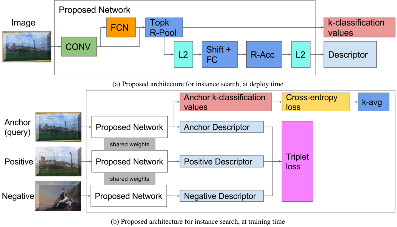
Figure 2: Proposed architecture for instance search, based on an FCN [17] for region proposals.
