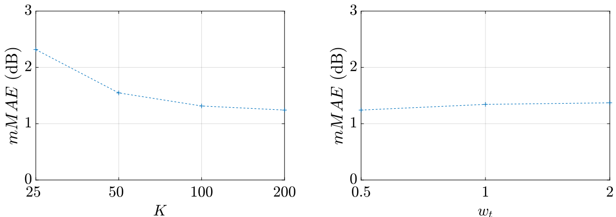
(a) Influence of the experimental factor \mathbf{K} (TI-NMF, w_t = 0.5 s, \beta = 2 , t_h = 0.32 , 400 iterations).
