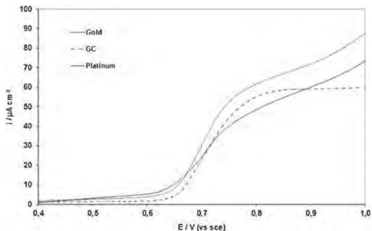
Fig. 3 Rotating disk electrode for vanillin oxidation at 5.10^{-5} mol L ^{-1} on gold, GC, and platinum electrodes in a phosphate buffer solution at pH=5.0
