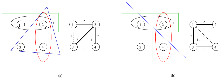
Fig. 2: Example of a hypergraph (a) with a feasible solution tree and (b) without a feasible solution tree
