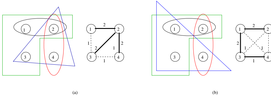
Fig. 2: Example of a hypergraph (a) with a feasible solution tree and (b) without a feasible solution tree
