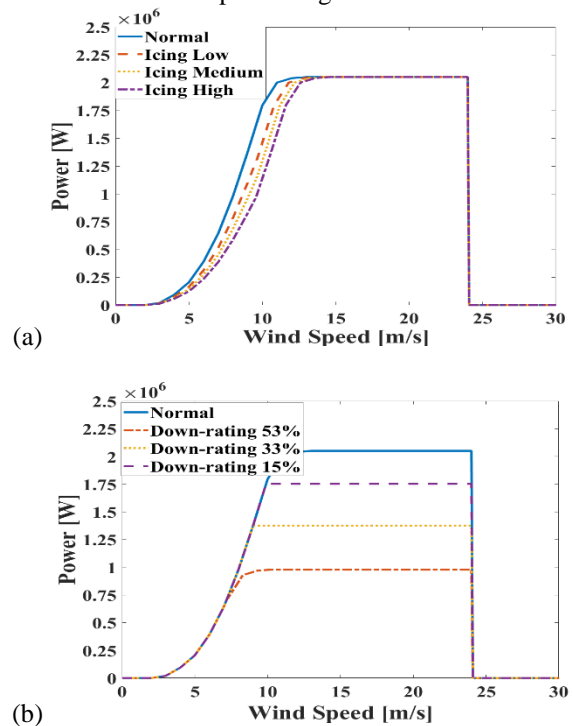
Figure 3. Fault Reference Power Curves for (a) Icing & (b) Down-rating
