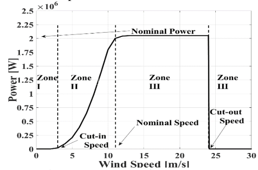
Figure 1. Example of a power curve
