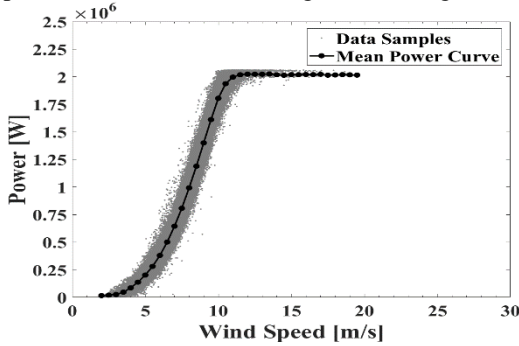
Figure 4. Real Power Curve Data for dispersion learning
