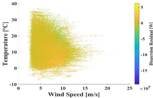
Figure 5. Learnt Dispersion Residual (w.r.t wind speed & Temperature)
