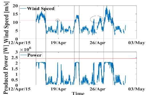
Figure 7. (a) Input Real Wind Profile & (b) Corresponding Simulated Power Profile
