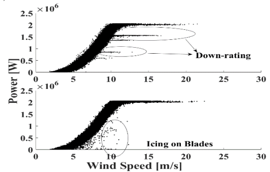
Figure 2. Types of power curves in various failures (a) Down-rating & (b) Icing on blades
