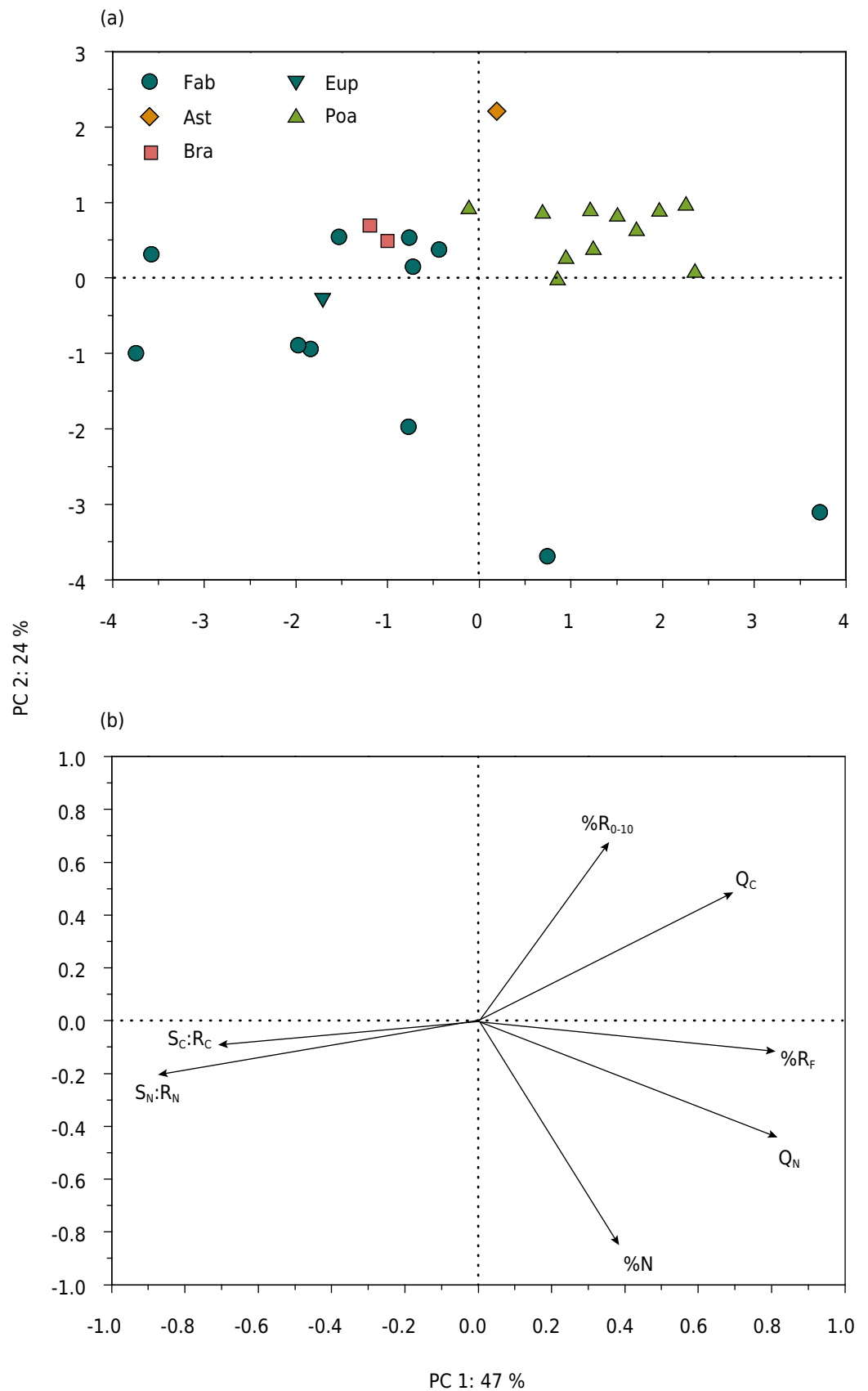
Figure 3. Factorial map (PC 1 \times PC 2) (a) and correlation circle (b) obtained from principal component analysis (PCA) performed using data from the roots of 27 species: vertical distribution ( \%R_{0.00-0.10} ), proportion of fine roots ( \%R_F ), root C and N contents ( Q_C , Q_N ), root N concentration ( \%N ), and shoot:root ratio for N and C inputs ( S_N:R_N and S_C:R_C ). Fab = Fabaceae; Poa = Poaceae; Ast = Asteraceae; Bra = Brassicaceae; Eup = Euphorbiaceae.
