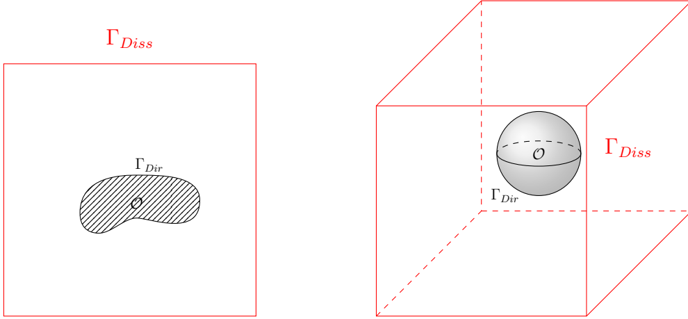
FIGURE 1. Examples of domains with an obstacle satisfying Assumptions 1 and 2 with \Gamma_{Diss} convex
