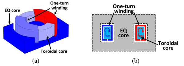
Fig. 3. T-EQ CM choke model for simulation. (a) One-turn equivalent model. (b) Cross section view.
