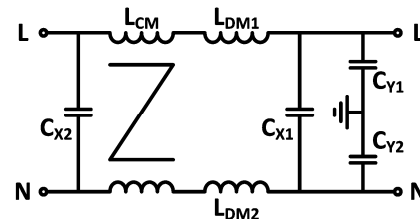
Fig. 1. Typical topology of EMI filter
