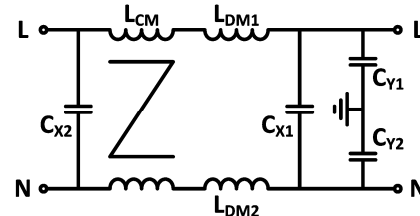
Fig. 1. Typical topology of EMI filter
