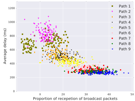
Figure 13. Impact of the number of broadcast rate on the end-to-end delay.
