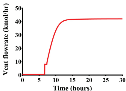
Fig. 18. Vent flowrate established in the column C-2 for the scenario 8.
