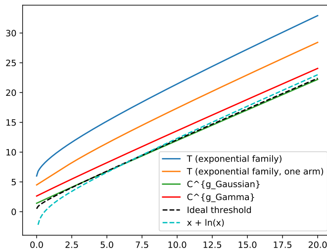
Figure 2: Several threshold functions \mathcal{C}(x) as a function of x .
