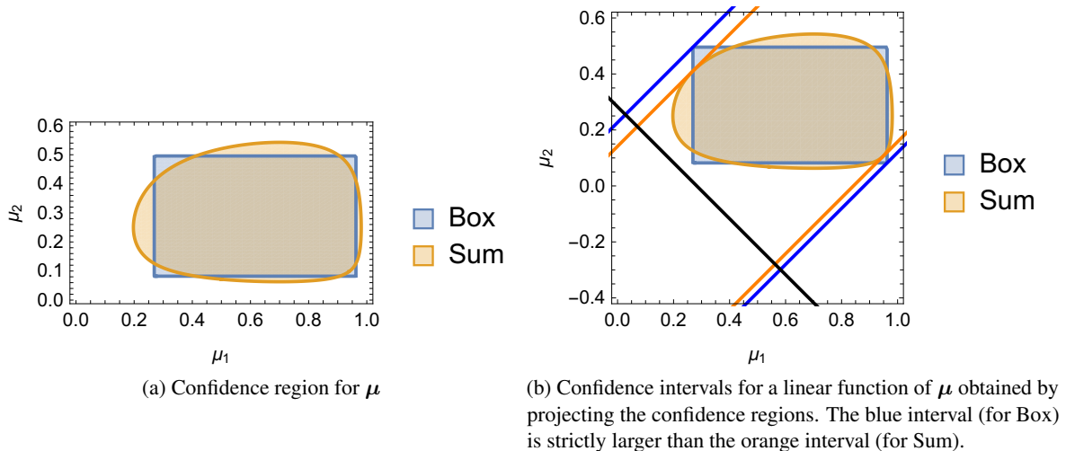
Figure 1: Visual two-arm comparison of confidence regions and implied confidence intervals. A union bound over traditional per-arm confidence intervals gives the “Box” region. Our new bound (2) results in a confidence region of the egg-shape marked “Sum”.
