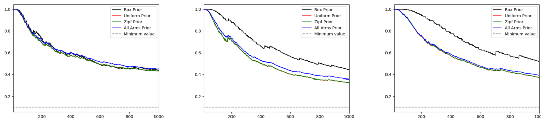
Figure 4: U_t^{\tilde{\pi}}(\delta) as a function of t for several cardinality-based priors \tilde{\pi} in a presence of M = 1 (left), M = 5 (middle) and M = 10 (right) identical arms with minimal expectation.
