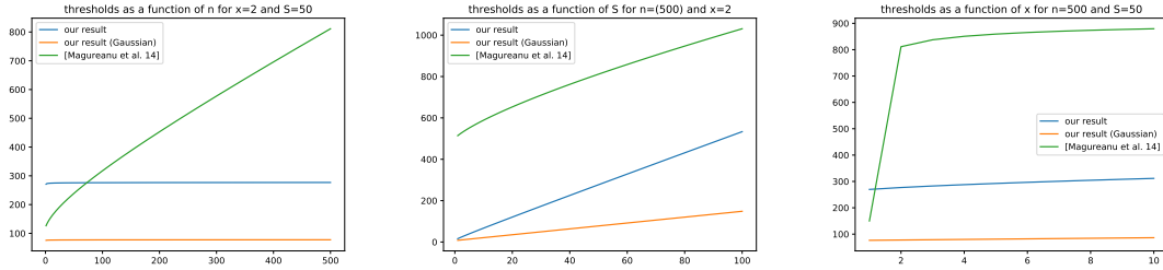
Figure 3: Thresholds that follow from Corollary 12 and Theorem 16 compared to that obtained by Magureanu et al. (2014)
