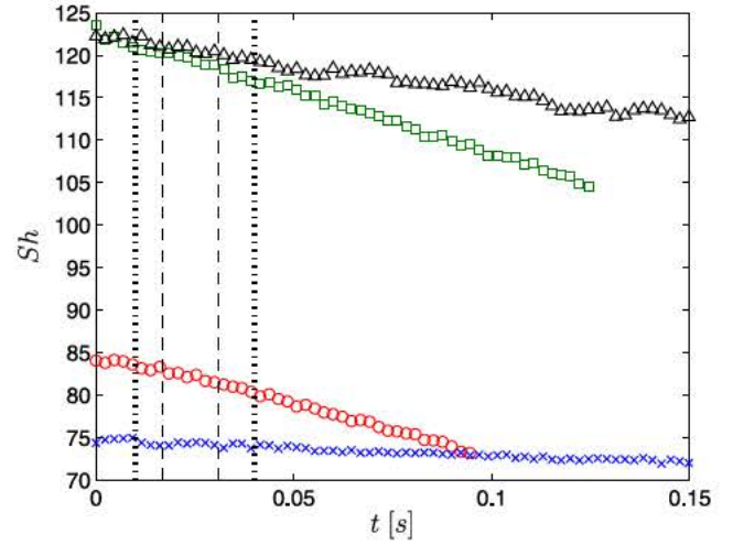
Fig. 11. Bubble sherwood number evolution versus time for \times T 30 °C, \Delta T 50 °C, \square T 100 °C, \circ T 150 °C, - - \tau_D \approx 17 –31 ms, ... 5\tau_v 10–40 ms.
