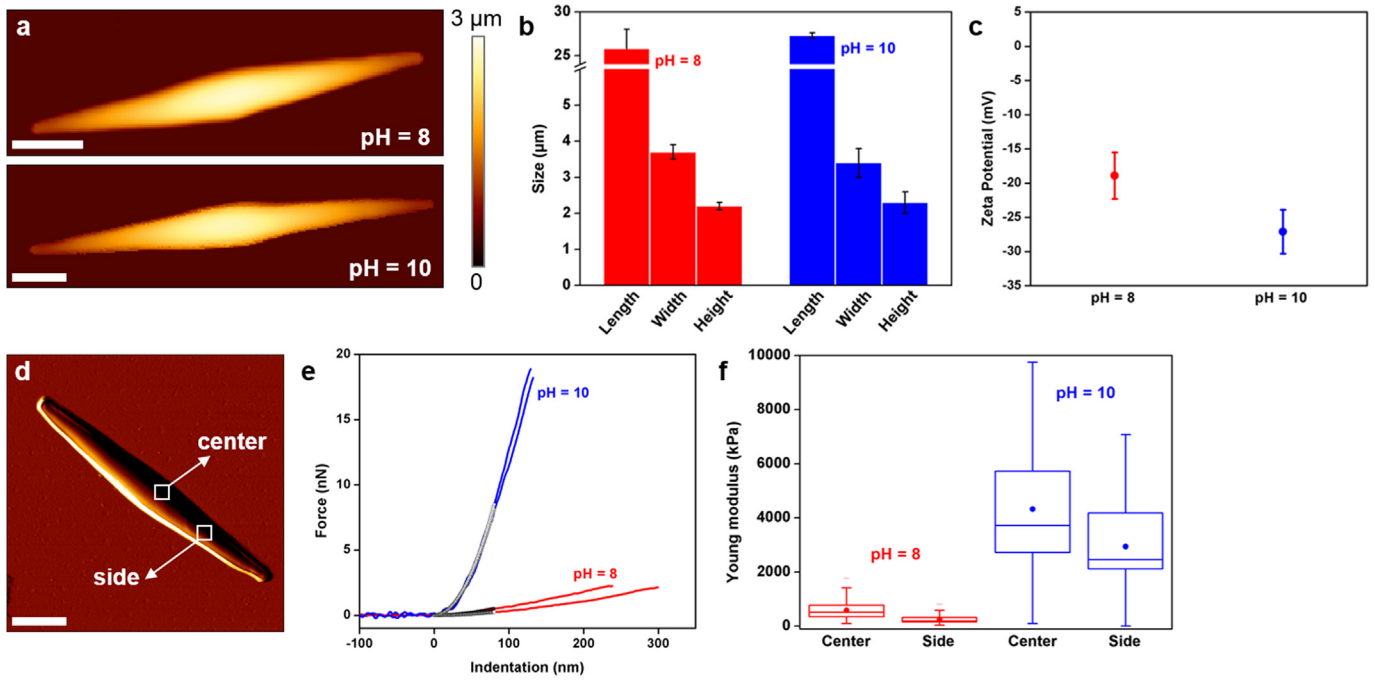
Fig. 2. Morphology and surface properties of cells at different pH. (a) AFM height images of P. tricorutum cells in sorbitol buffer at pH = 8 or pH = 10. (b) Histogram representing the length, width and height of cells at pH = 8 or pH = 10. For each conditions, 6 cells coming from 2 independent cultures were analyzed. (c) Zeta potential of cells in sorbitol buffer as a function of the pH. For each pH, 15 independent measurements were performed. (d) AFM vertical deflection image of a single P. tricorutum cells in sorbitol buffer at pH = 10. Squares indicate 1 μm × 1 μm areas where local nano-indentation measurements were performed. (e) Representative indentation curves recorded on the center or the side of cells at pH = 8 or pH = 10. Black empty circles on the curves represent the Hertz model used to fit the curves and extract the Young modulus values (f) Box charts showing the distribution of Young modulus values obtained from curves recorded on the center or the side of cells in sorbitol buffer at pH = 8 or pH = 10. For each condition, 8192 curves recorded on 8 cells coming from 3 independent cultures were analyzed. Scale-bars in AFM images correspond to 5 μm.
