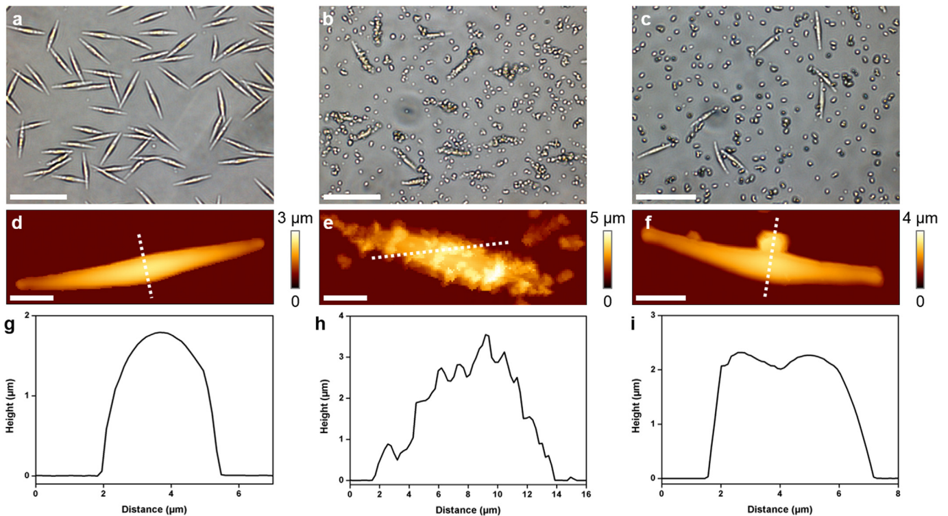
Fig. 3. Effects of flotation on P. tricorutum cell surface. (a) Optical image of cells before flotation in sorbitol buffer at pH = 10, or (b) after flotation in sorbitol buffer pH = 10 with Mg(OH) 2 at a concentration of 5.7 mM or (c) with Ca(OH) 2 at a concentration of 10.5 mM. (d) AFM height image of a single P. tricorutum cell before flotation, or (e) after flotation in sorbitol buffer pH = 10 with Mg(OH) 2 at a concentration of 5.7 mM or (c) with Ca(OH) 2 at a concentration of 10.5 mM. (g), (h) and (i) are cross-sections taken along the white dashed white lines in respectively (d), (e) and (f). Scale-bars in optical images correspond to 50 μm and to 5 μm in AFM images.
