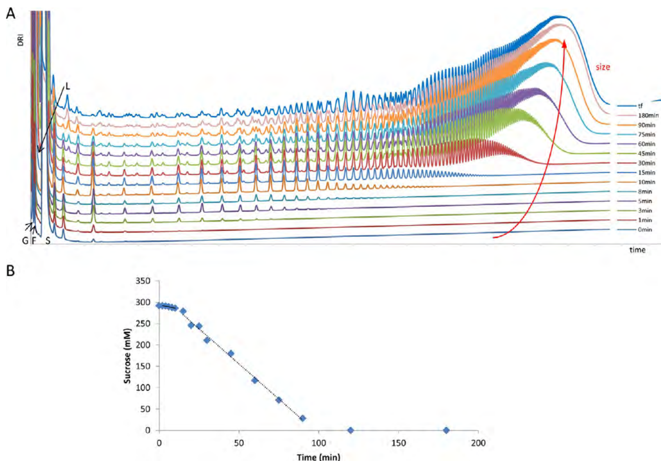
Figure 3. Monitoring of oligosaccharide and polysaccharide production during polymerization catalyzed by DSR-M \Delta 2: (A) HPAEC-PAD chromatograms during the polymerization reaction (G, glucose; F, fructose; S, sucrose; L, leucrose); (B) sucrose consumption during the reaction.
