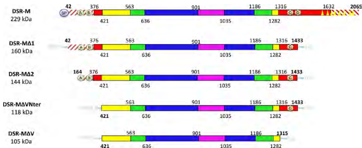
Figure 1. Schematic structural organization of DSR-M and the truncated variants, based on amino acid alignment with GTF-180- \Delta N and structural analysis. Hatched red lines correspond to nonaligned zones. DSR-M structural domains: (i) domain V in red; (ii) domain IV in yellow; (iii) domain A in blue; (iv) domain B in green; (v) domain C in magenta. The blue circle represents the signal peptide, APY motifs are indicated with triangles, and pale yellow stars marked as A–D represent putative glucan binding pockets.
