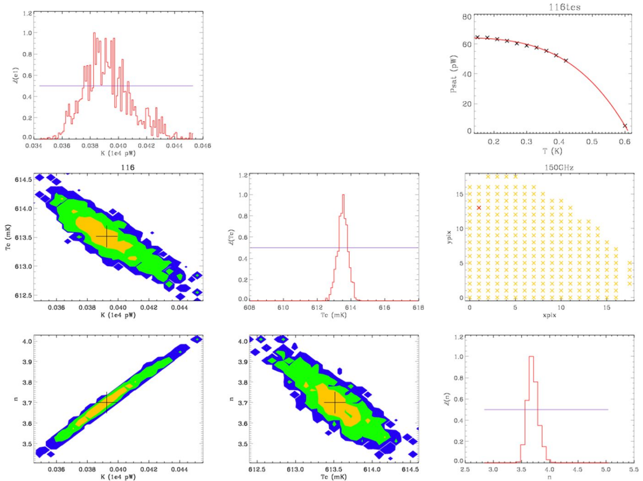
Figure 6: Parameters of a QUBIC TES estimated with a suitable MCMC algorithm developed for AdvACT 25 (color figure online). From top right to bottom left: experimental data and estimated theoretical fit, QUBIC detector array, TES parameters likelihoods and contour plots of the TES parameters.
