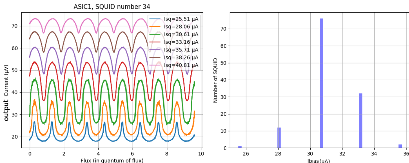
Figure 2: Left: typical current response of a QUBIC StarCRYO SQ600S SQUID (color figure online). Right: histogram of the SQUID response for each SQUID read out with ASIC1.
