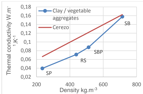
Fig. 6: Dry mortar thermal conductivities and densities of clay/vegetables samples
