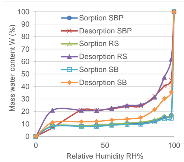
Fig. 8: SB, SBP and RS sorption/desorption isotherm
