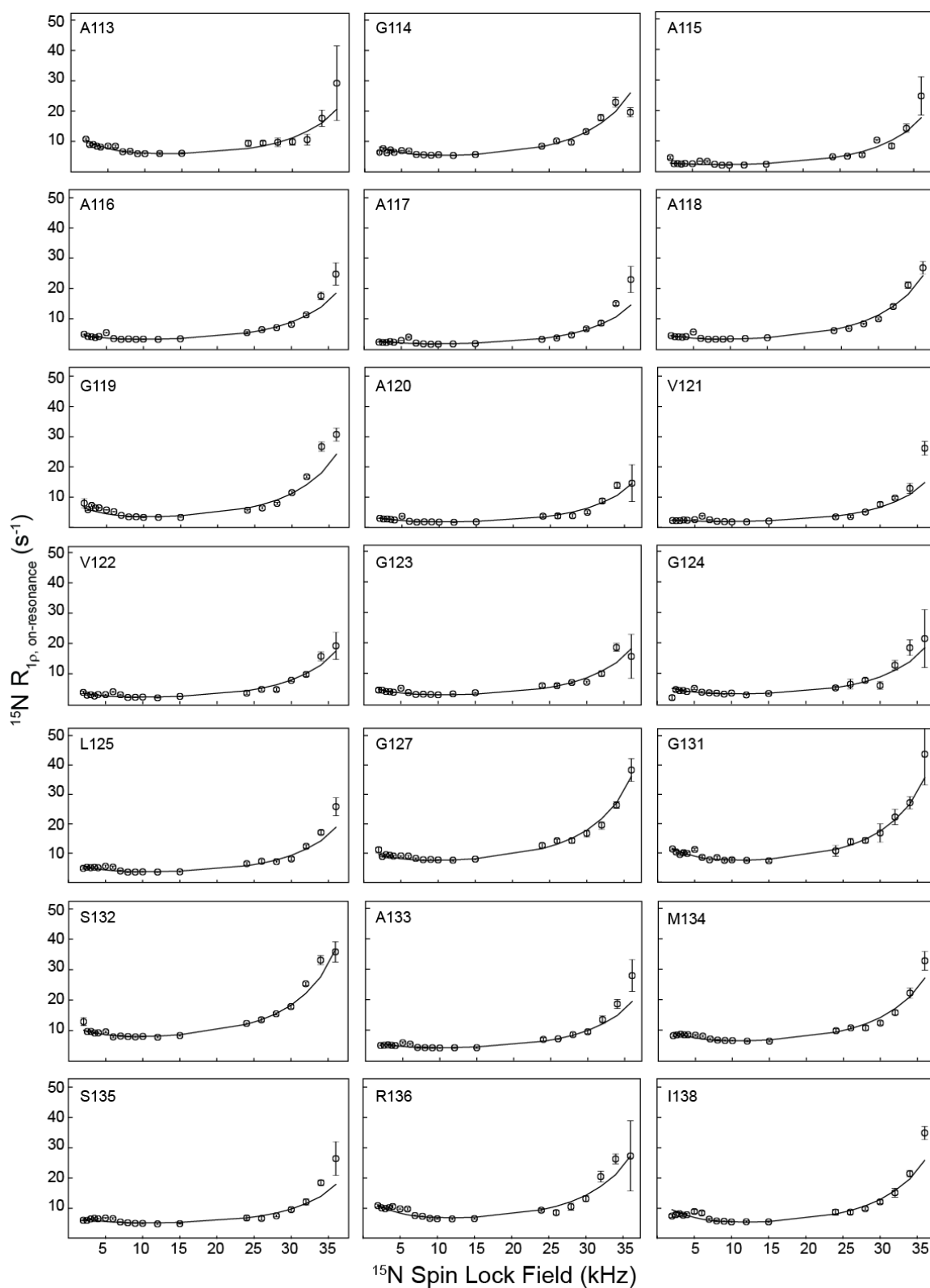
Figure 2. Residue-specific ^{15}\text{N} R_{1\rho} RD profiles for huPrP23-144 amyloid fibrils at 800 MHz ^1\text{H} frequency. Experimental data are shown as open circles, and numerical fits used to extract the global exchange rate and minor excited-state population, as well as site-specific parameters \Delta\omega and \alpha (c.f., Figure 3) are shown as solid lines. RD profiles for residues G126, L130, and F141, which were not fit as well by the global exchange model, are shown in SI Figure S5 along with individual residue-specific fits. RD profiles for residues I139 and H140 could not be obtained due to insufficient resolution in the 2D ^{15}\text{N} - ^1\text{H} spectrum.
