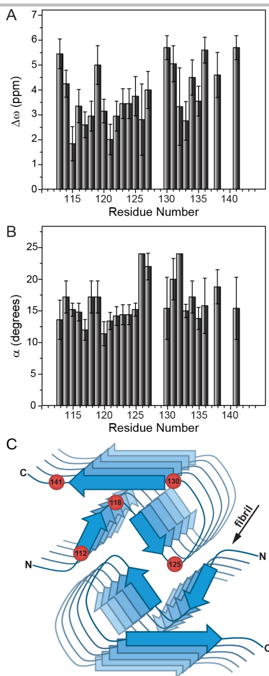
Figure 3. Plots of residue-specific (A) \Delta\omega and (B) \alpha values extracted from the global fit of ^{15}\text{N} R_{1\rho} RD profiles for huPrP23-144 amyloid with k_{\text{ex}} = 1,000\text{ s}^{-1} and p_{\text{B}} = 2\% . (C) Schematic structural model of the huPrP23-144 fibril with approximate locations of several amino acid residues indicated by red spheres.
