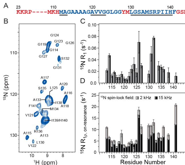
Figure 1. (A) Amino acid sequence of huPrP23-144, with the most rigid amyloid core residues shown in blue font. The dynamically disordered N- and C-terminal residues and two flexible residues located within the core region, which are not detectable in conventional solid-state NMR experiments, are shown in red font. Regions with the highest \beta -strand propensity predicted by TALOS-N [37] based on backbone ^{13}\text{C} and ^{15}\text{N} chemical shifts are underlined. (B) 2D ^{15}\text{N} - ^1\text{H} chemical shift correlation spectrum of amyloid fibrils generated from ^2\text{H} , ^{13}\text{C} , ^{15}\text{N} -labeled huPrP23-144 back-exchanged in a 1:1 mixture of \text{H}_2\text{O} and \text{D}_2\text{O} . The spectrum was recorded in 2 h at 800 MHz ^1\text{H} frequency, 40 kHz MAS rate, and sample temperature of \sim 10 ^\circ\text{C} . Due to large variations in resonance intensities, for clarity the cross-peaks are drawn with the lowest contour at 75 times the rms noise level. The locations of cross-peaks for residues A113, G124, G126, and L130, for which the signal-to-noise is below this threshold, are indicated. (C) Residue-specific ^{15}\text{N} R_1 values determined using the pulse sequence shown in SI Figure S2B. (D) Residue-specific ^{15}\text{N} R_{1\rho} values determined using the pulse sequence shown in SI Figure S2A with ^{15}\text{N} spin-lock fields of 2 kHz or 15 kHz as indicated.
