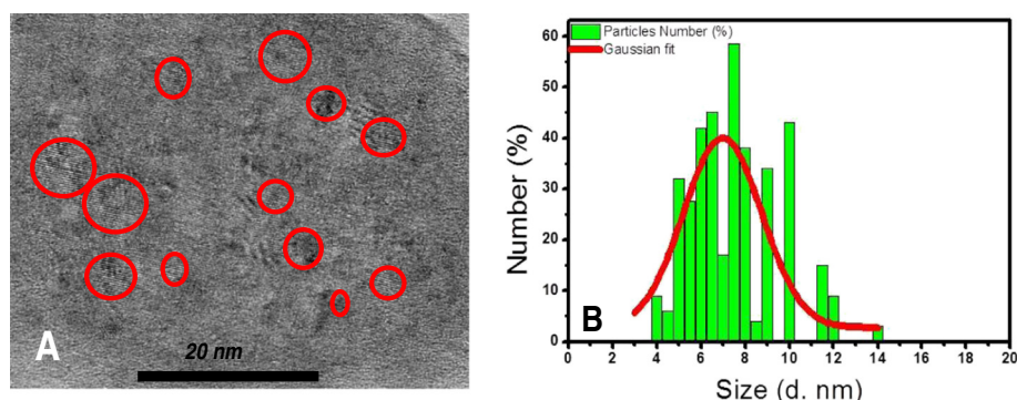
Figure 1 Transmission electron microscopy image and DLS measurement. (A) TEM image of Si powder initially suspended in ethanol and deposited on a graphite grid. (B) DLS of functionalized Si NPs dispersed in squalane.
