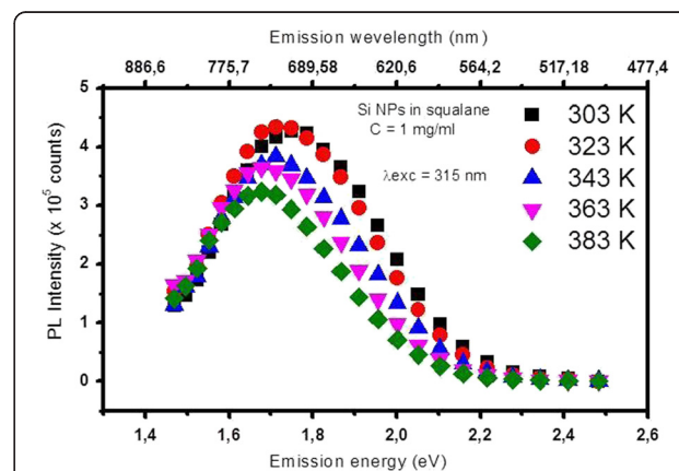
Figure 3 Temperature-dependent fluorescence spectra of Si NP colloidal suspension in squalane with a concentration of 1 mg/mL.
