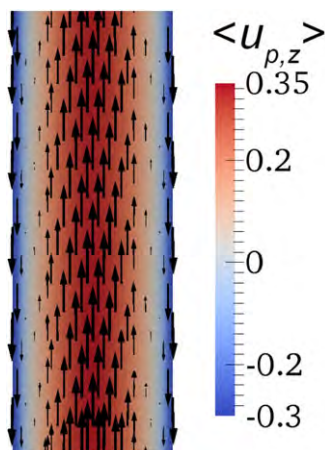
Figure 3. Time-averaged solid velocity vectors and solid vertical velocity field in background, in the tube region between 1.3 and 1.4 m (Ref case).
