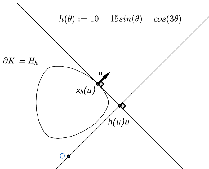
Figure 1. Envelope parametrized by its Gauss map
